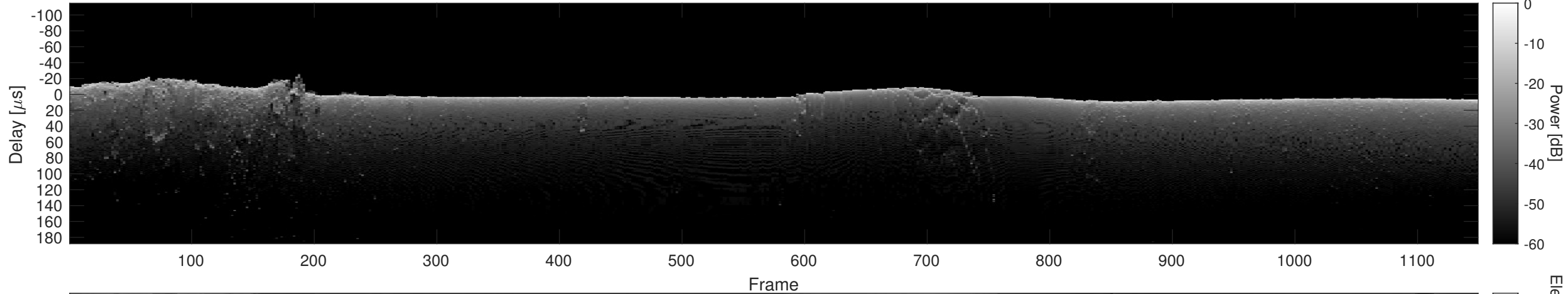
Orbit 18232, Cluttergram
