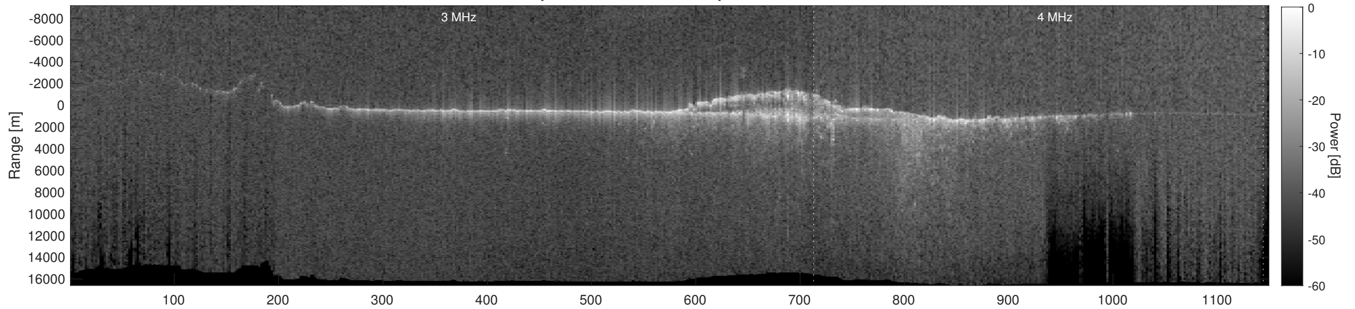
Orbit 18232, Depth-Corrected Cluttergram
