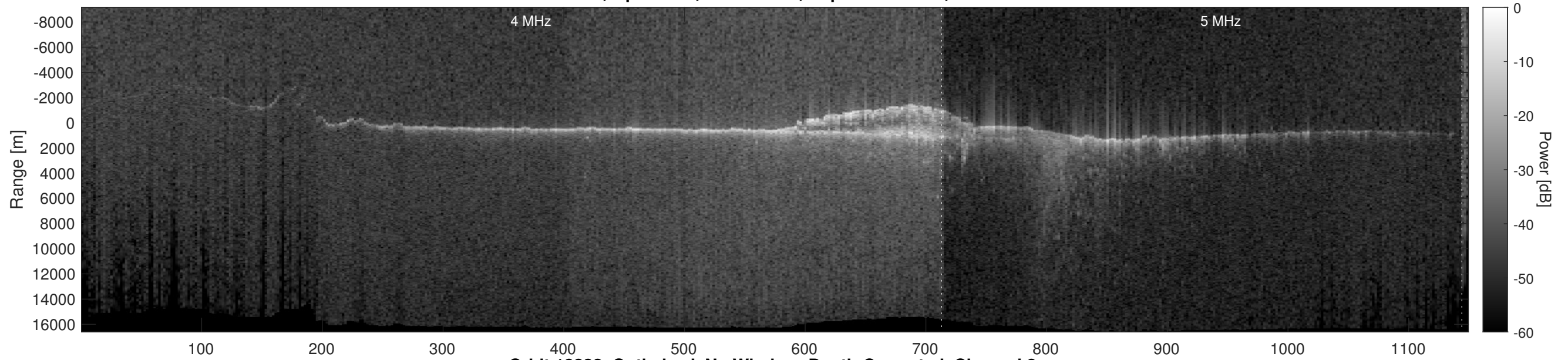
Orbit 18232, Optimized, No Window, Depth-Corrected, Channel 2
