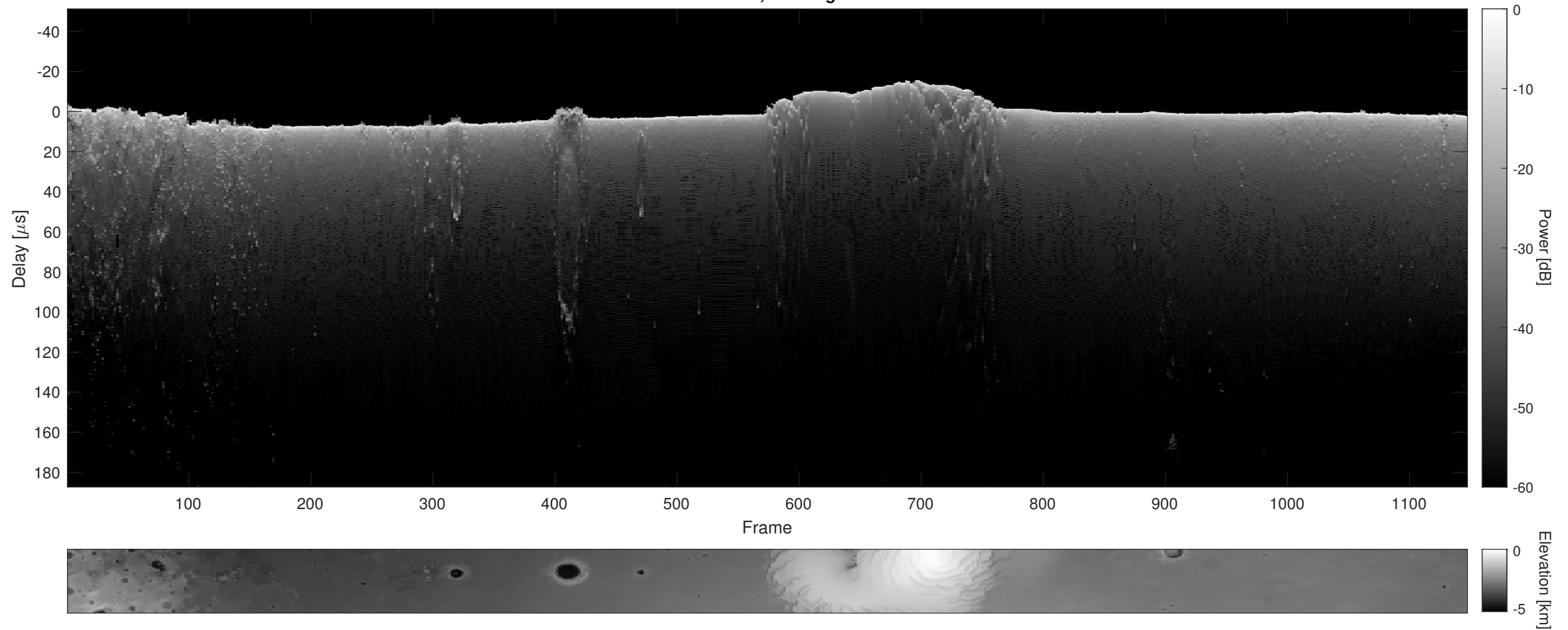
Orbit 18236, Cluttergram
