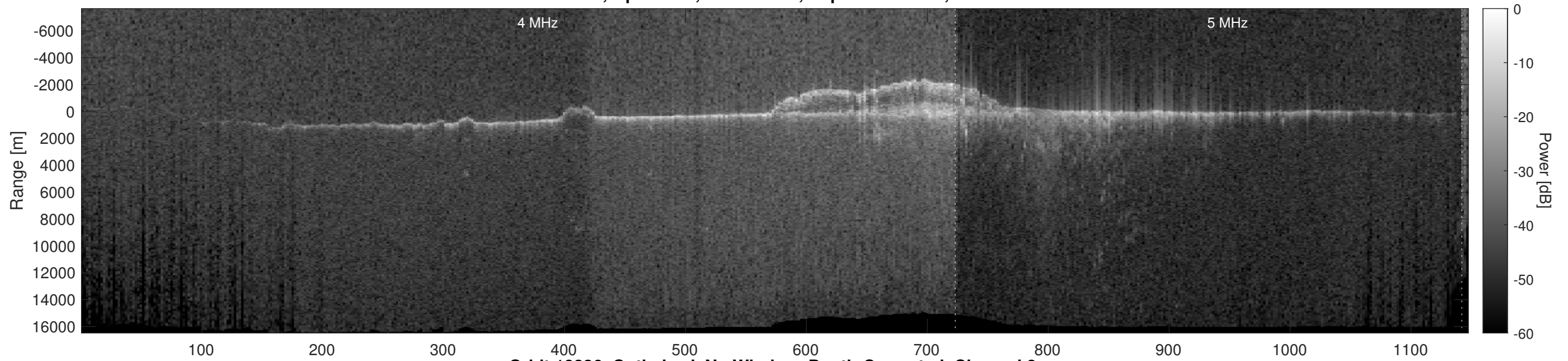
Orbit 18236, Optimized, No Window, Depth-Corrected, Channel 2
