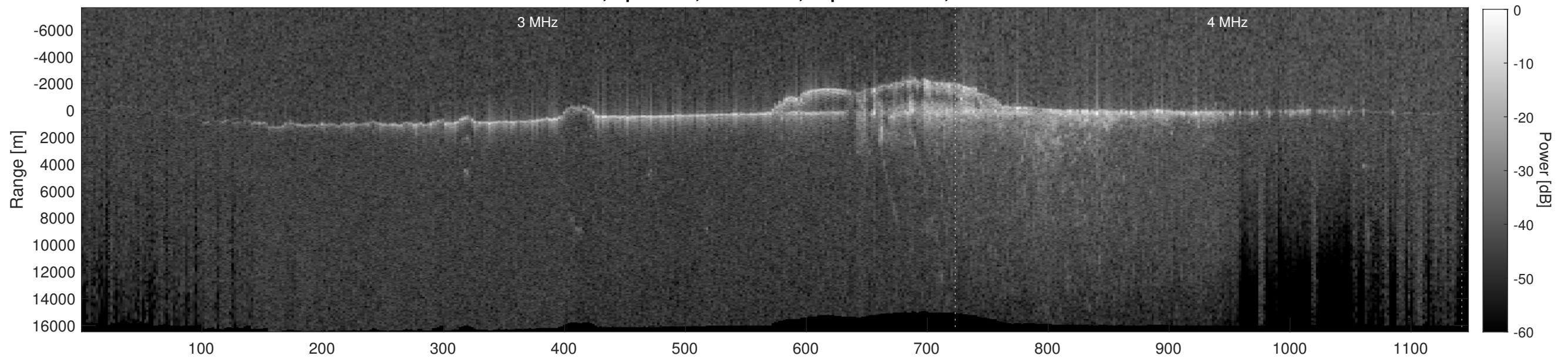
Orbit 18236, Depth-Corrected Cluttergram
