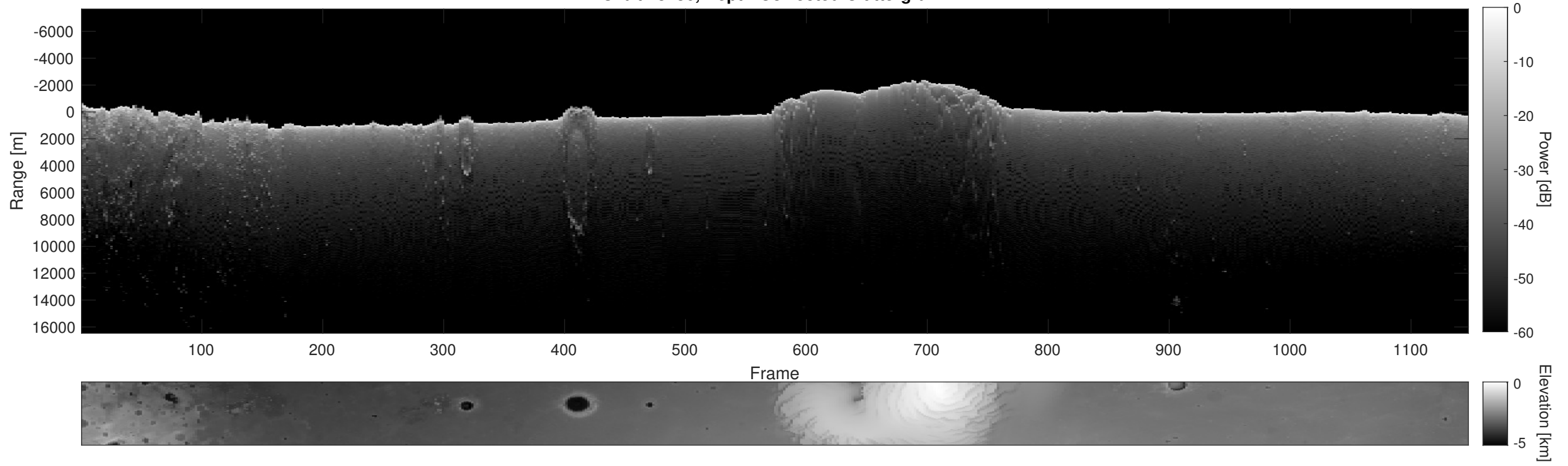
Orbit 18236, Depth-Corrected Cluttergram
