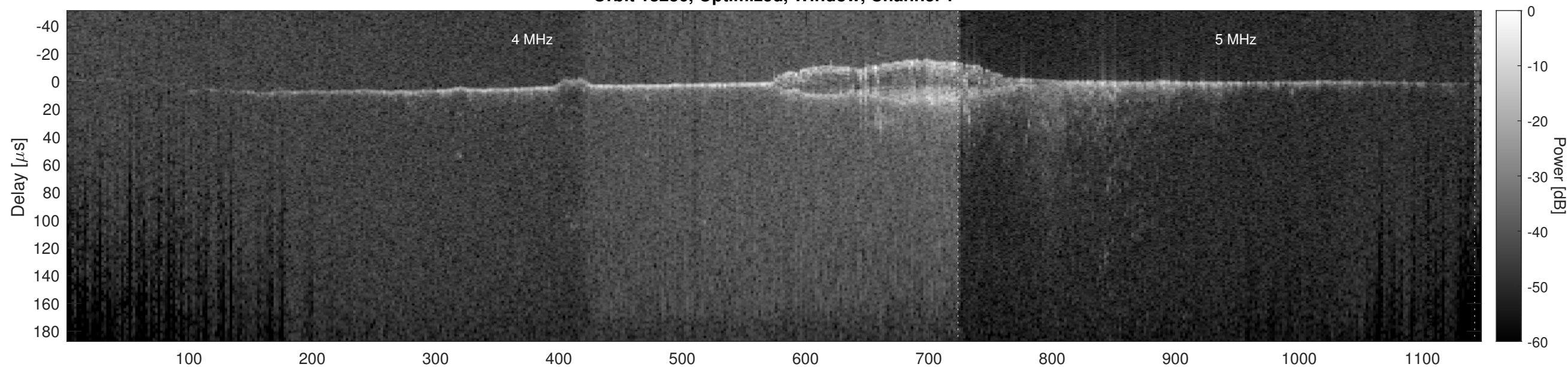
Orbit 18236, Optimized, Window, Channel 2
