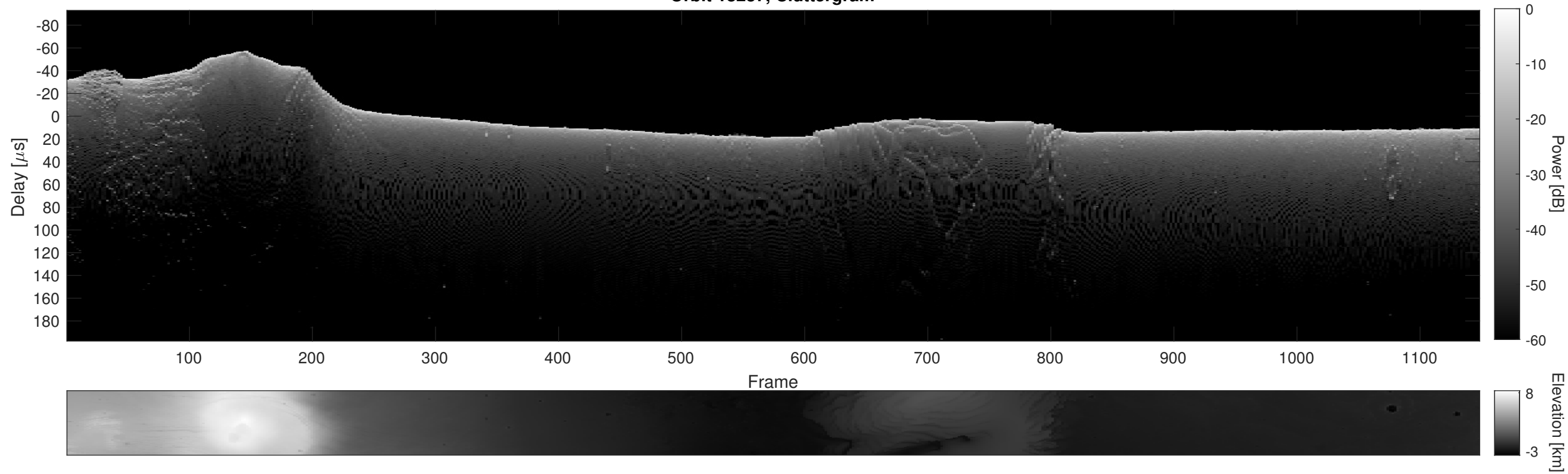
Orbit 18237, Cluttergram
