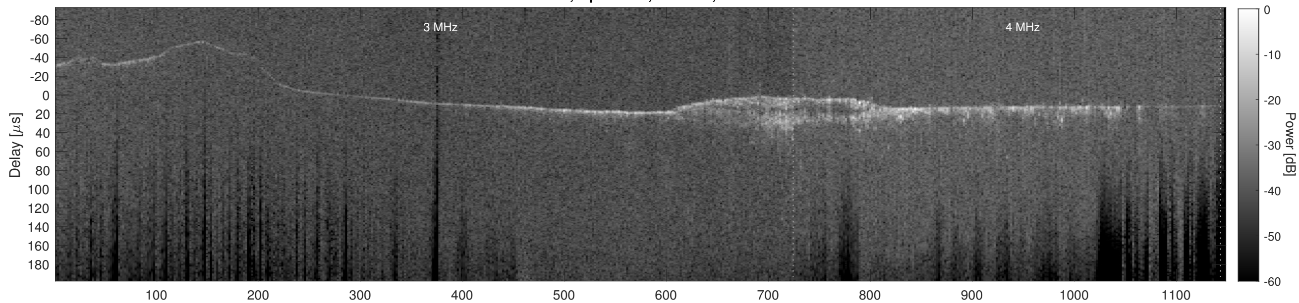
Orbit 18237, Cluttergram
