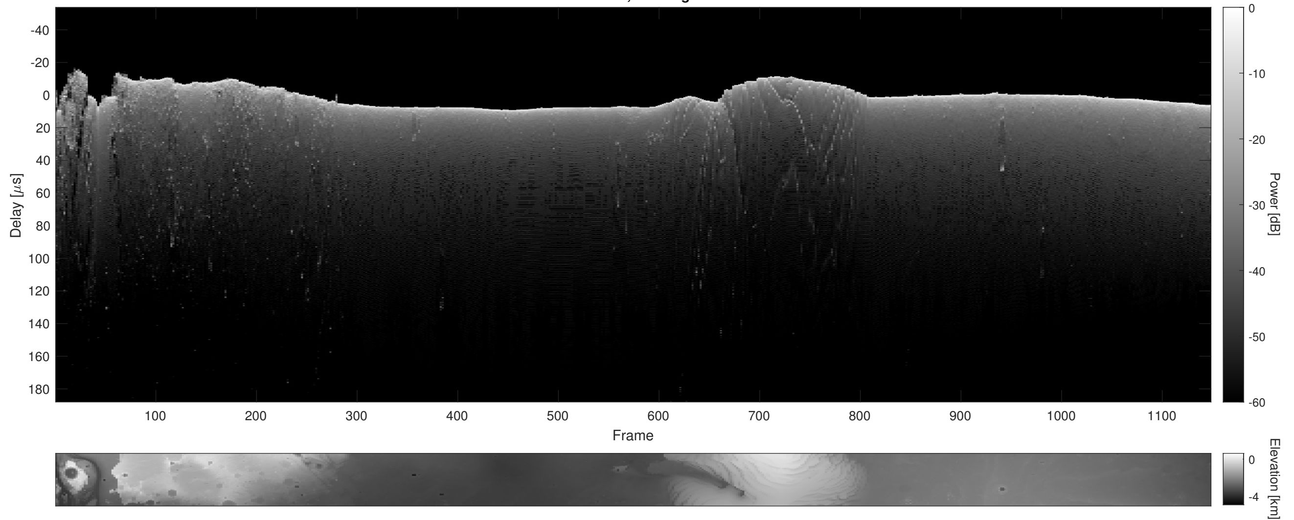
Orbit 18240, Cluttergram
