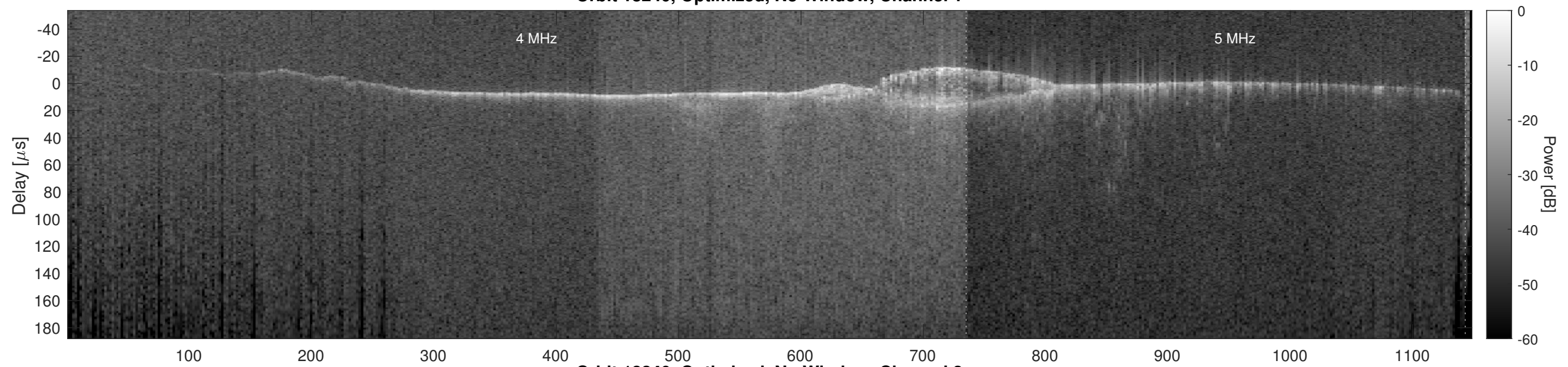
Orbit 18240, Optimized, No Window, Channel 2
