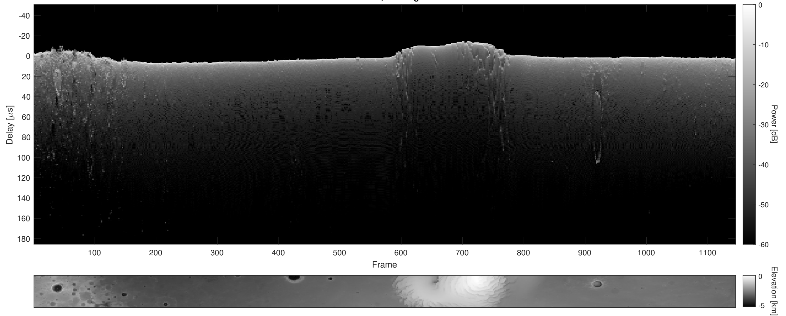
Orbit 18243, Cluttergram
