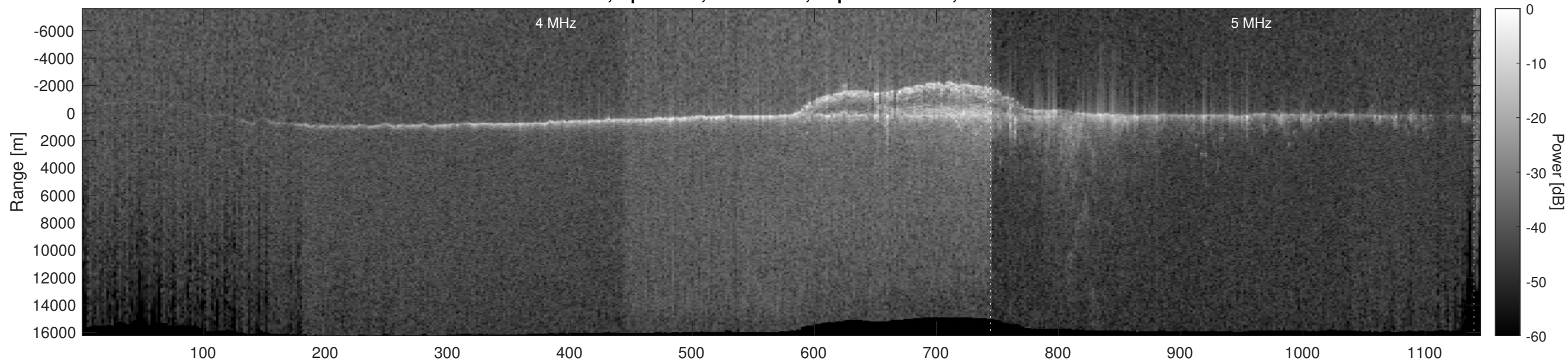
Orbit 18243, Optimized, No Window, Depth-Corrected, Channel 2
