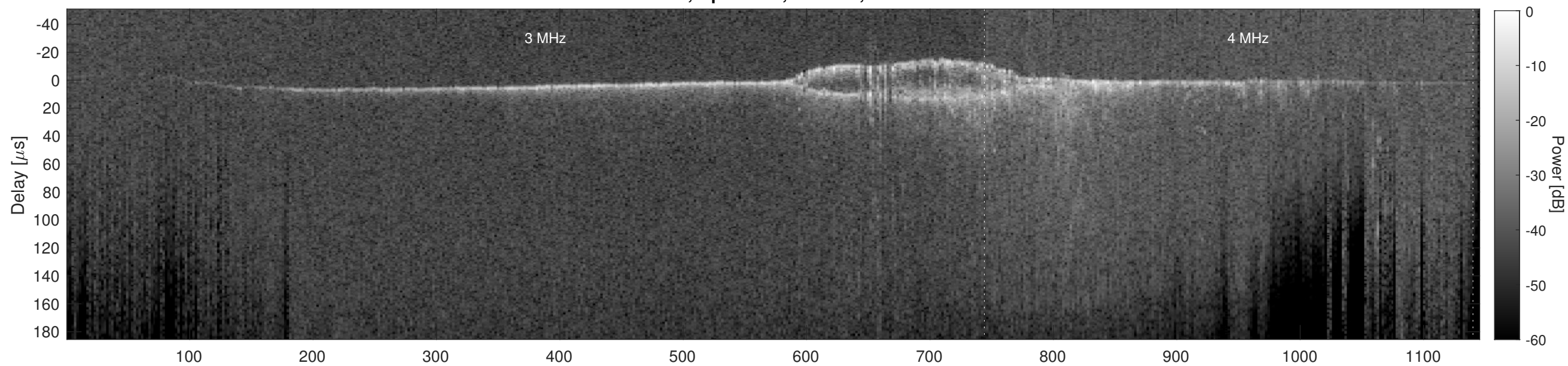
Orbit 18243, Cluttergram
