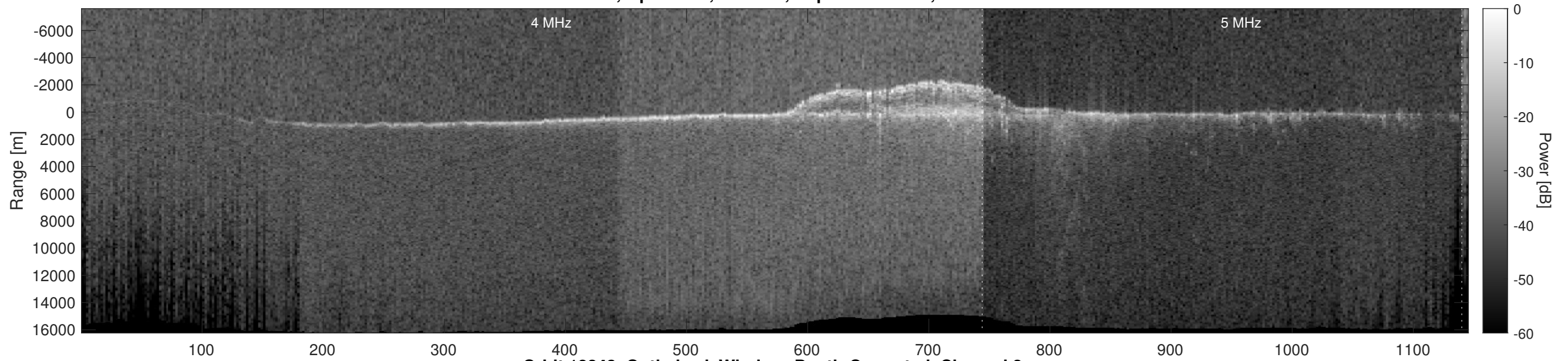
Orbit 18243, Optimized, Window, Depth-Corrected, Channel 2
