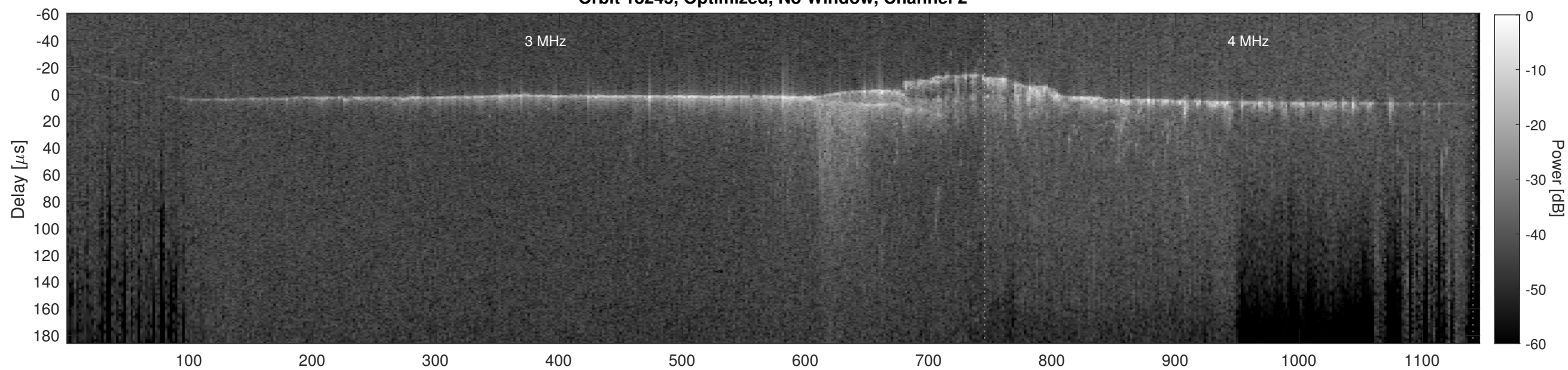
Orbit 18245, Cluttergram
