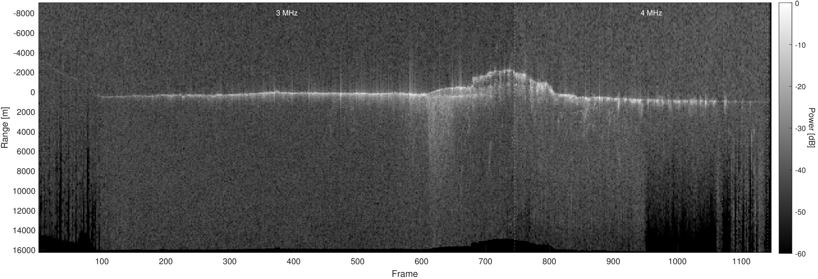
Orbit 18245, Optimized, No Window, Depth-Corrected, Channel 2
