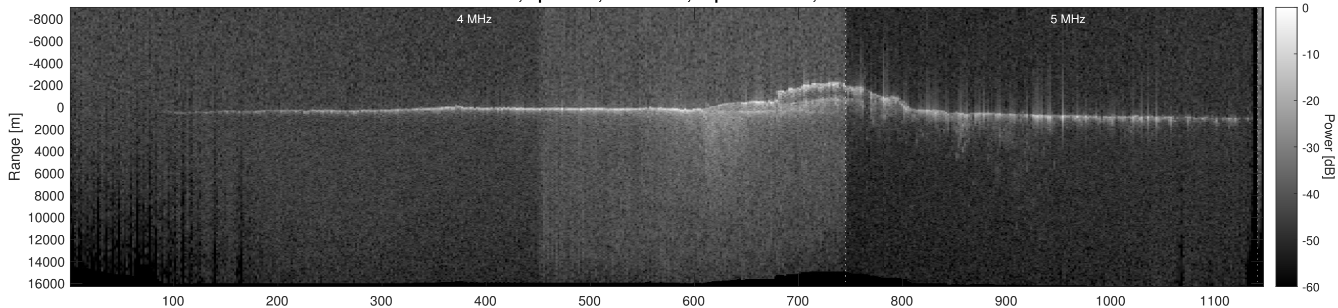
Orbit 18245, Optimized, No Window, Depth-Corrected, Channel 2
