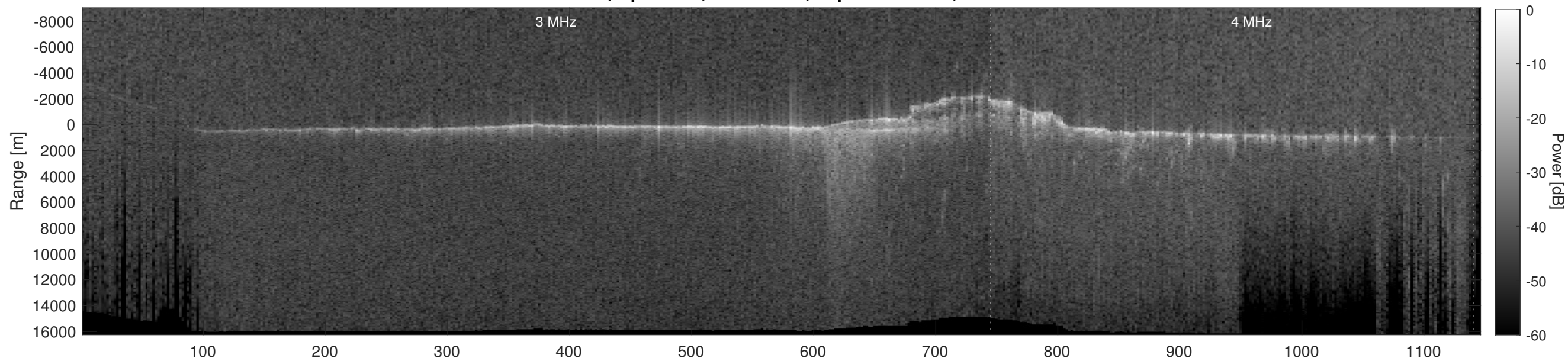
Orbit 18245, Depth-Corrected Cluttergram
