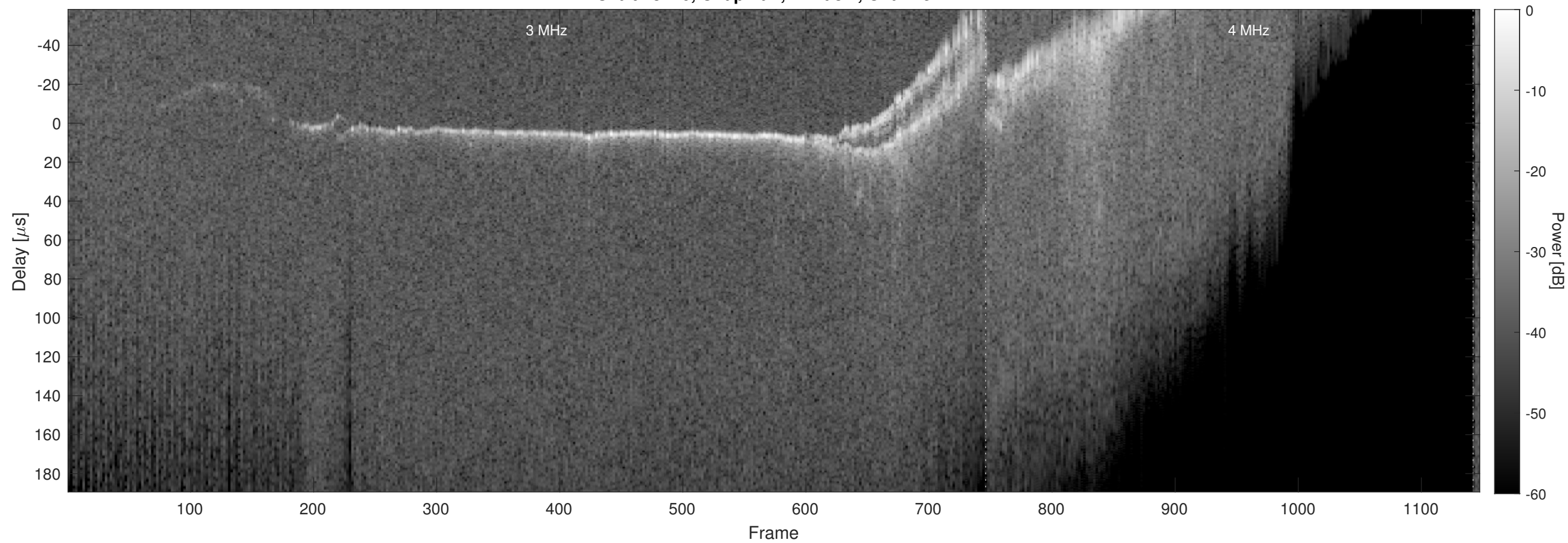
Orbit 18246, Chapman, Window, Channel 2
