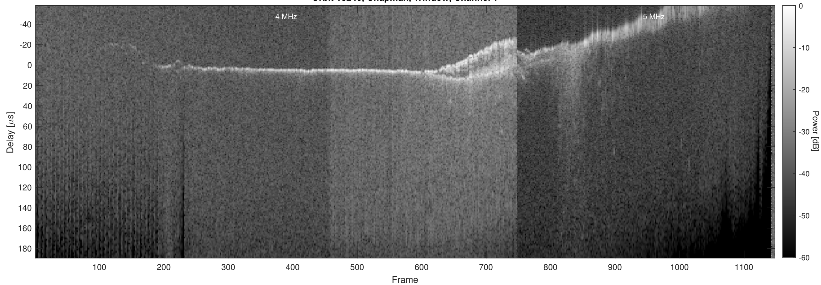
Orbit 18246, Chapman, Window, Channel 2
