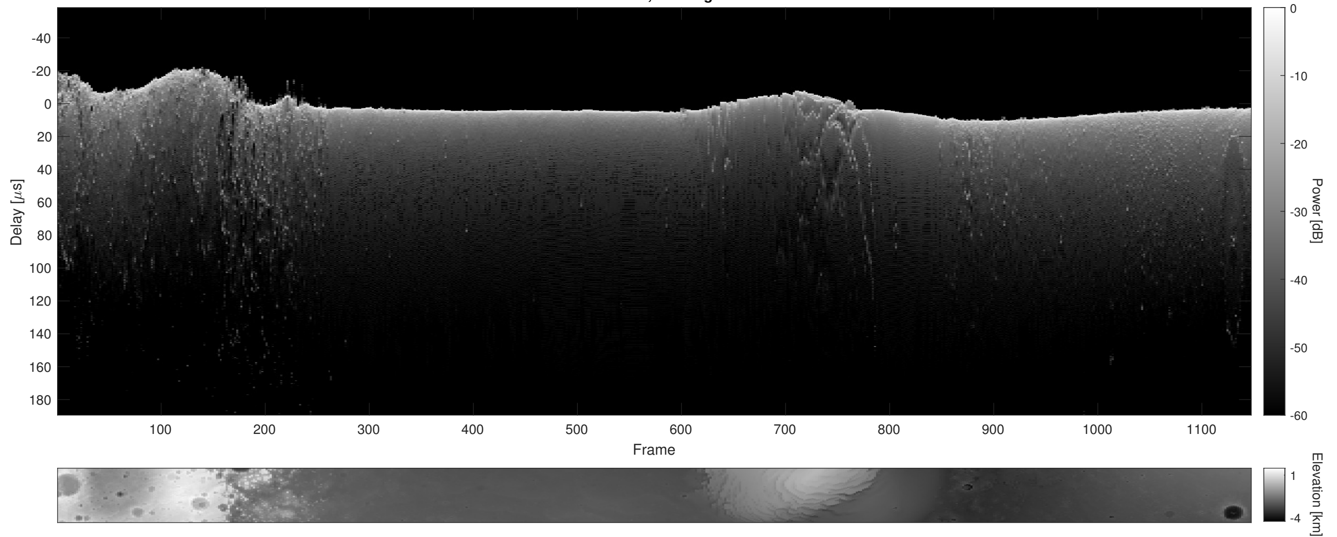
Orbit 18246, Cluttergram
