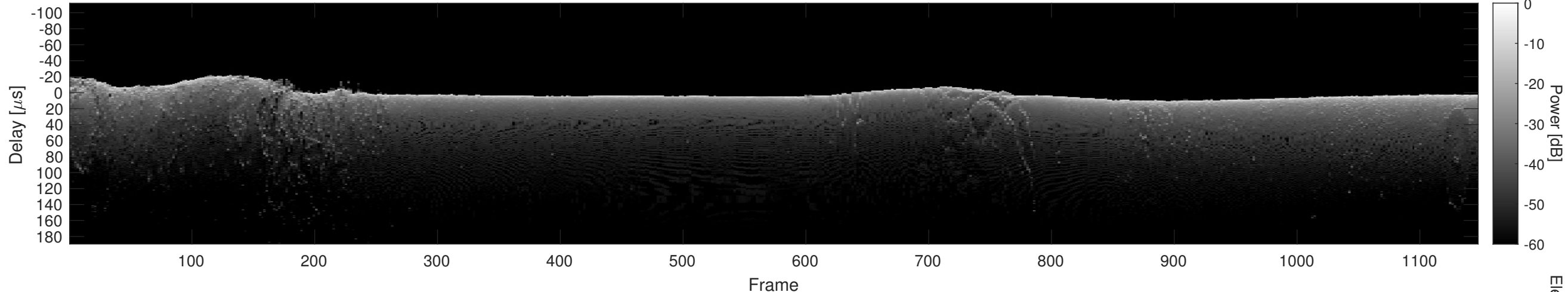
Orbit 18246, Cluttergram
