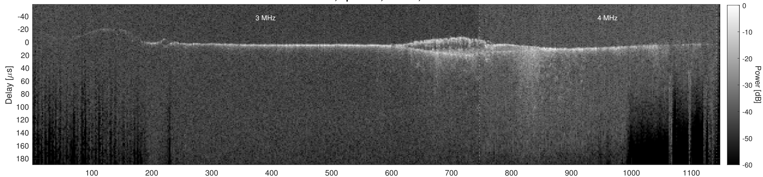
Orbit 18246, Cluttergram
