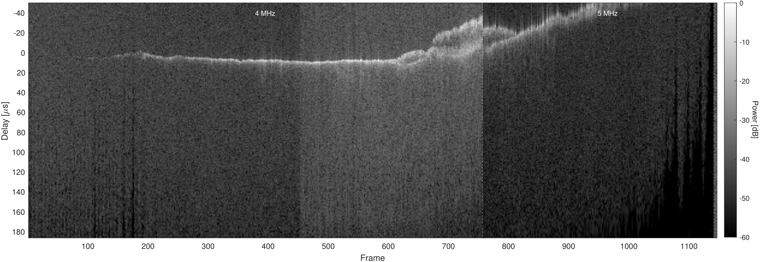
Orbit 18247, Chapman, No Window, Channel 2
