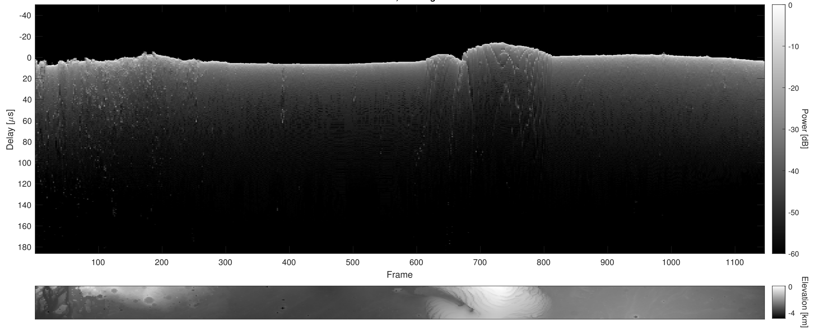
Orbit 18247, Cluttergram
