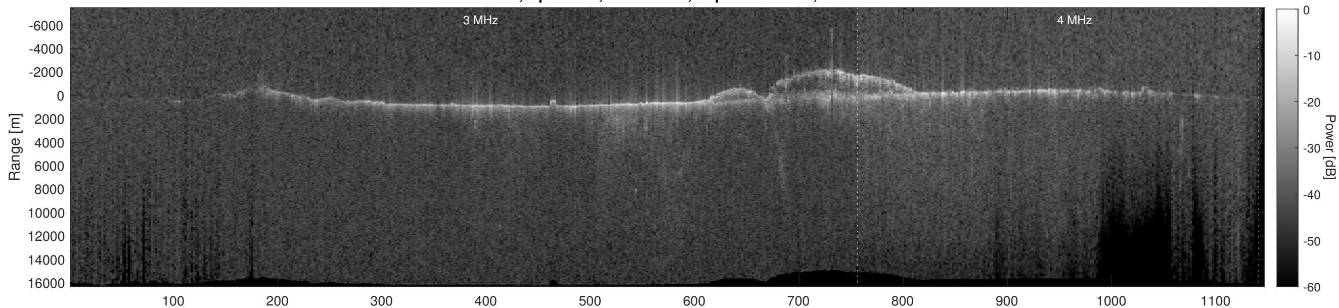
Orbit 18247, Depth-Corrected Cluttergram
