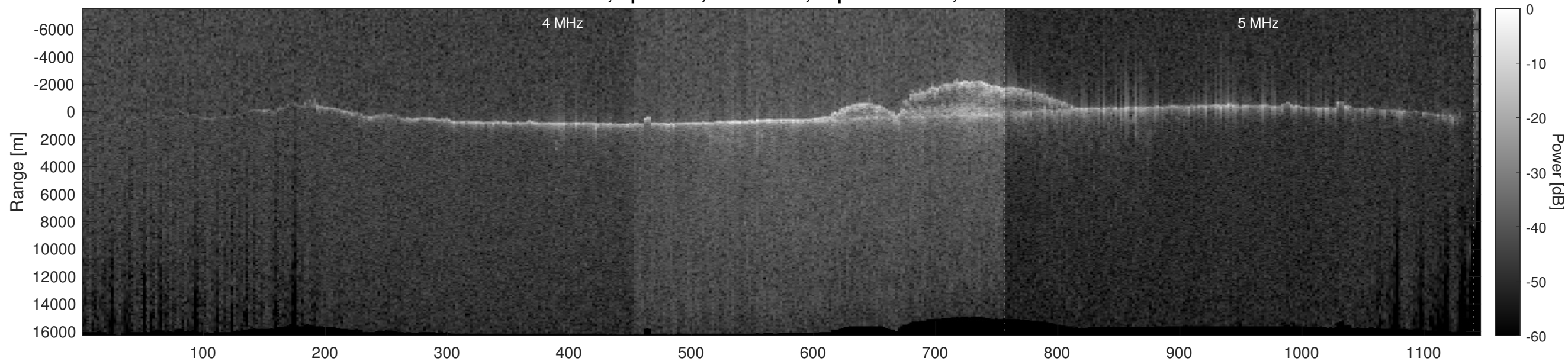
Orbit 18247, Optimized, No Window, Depth-Corrected, Channel 2
