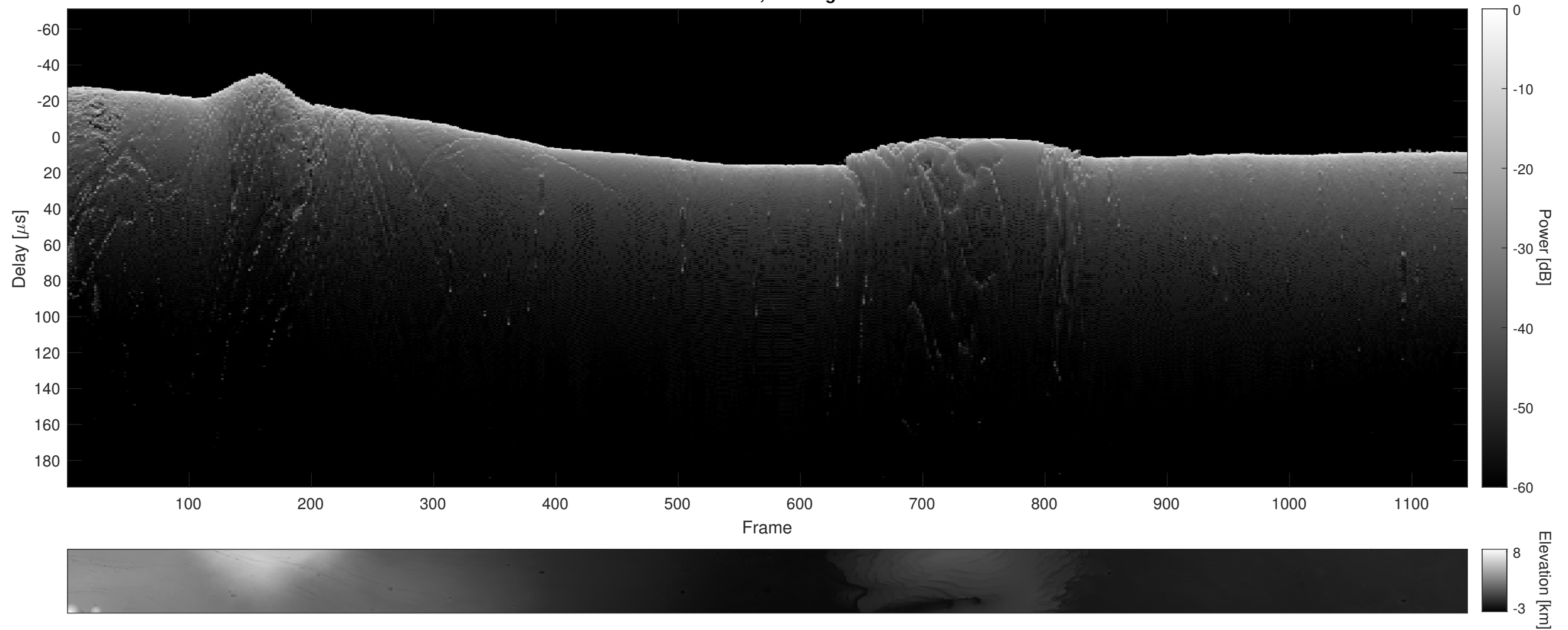
Orbit 18251, Cluttergram
