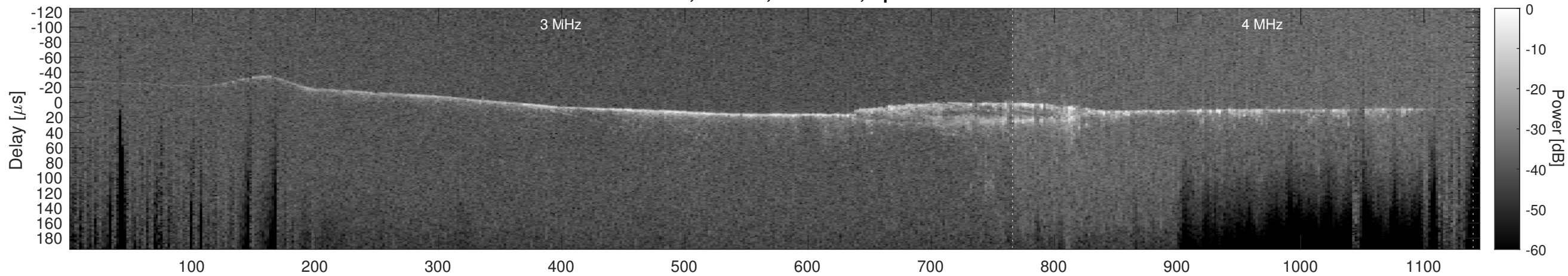
Orbit 18251, Cluttergram
