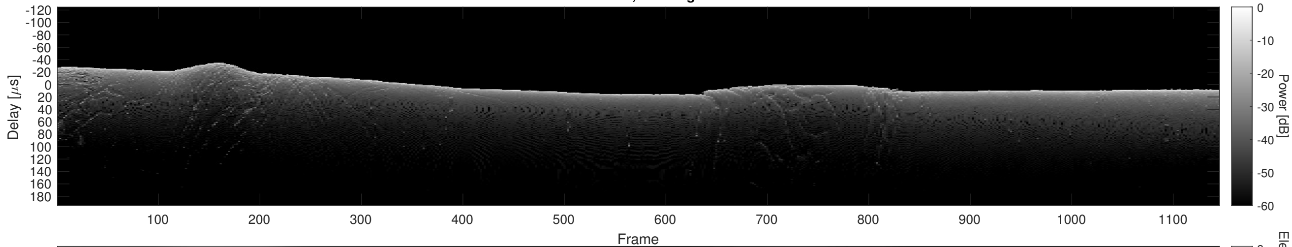
Orbit 18251, Cluttergram
