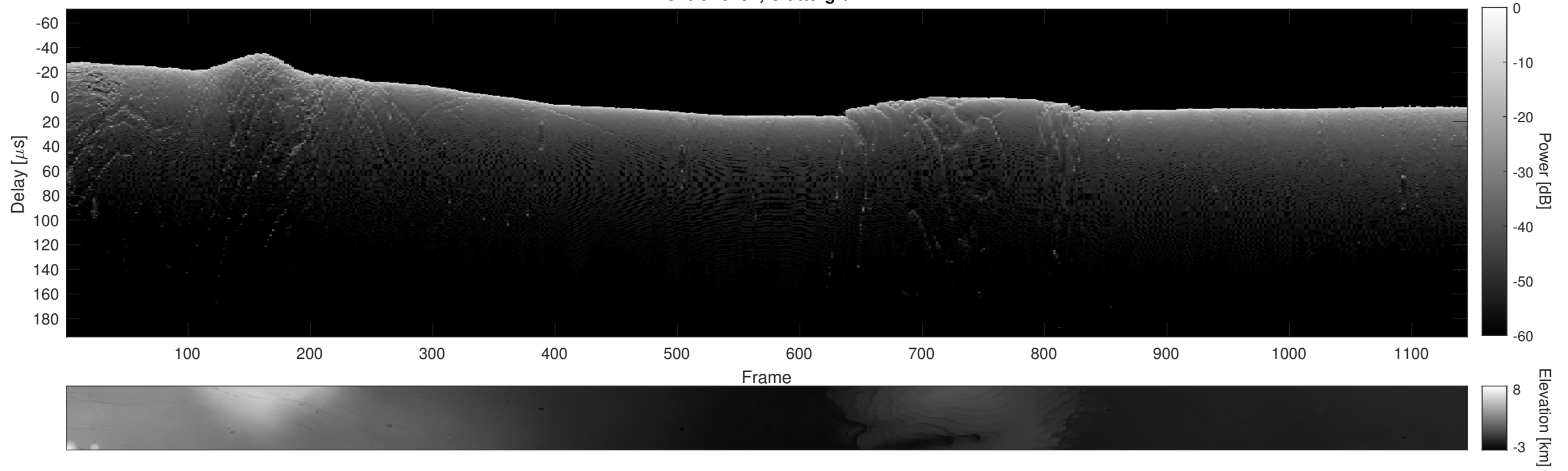
Orbit 18251, Cluttergram
