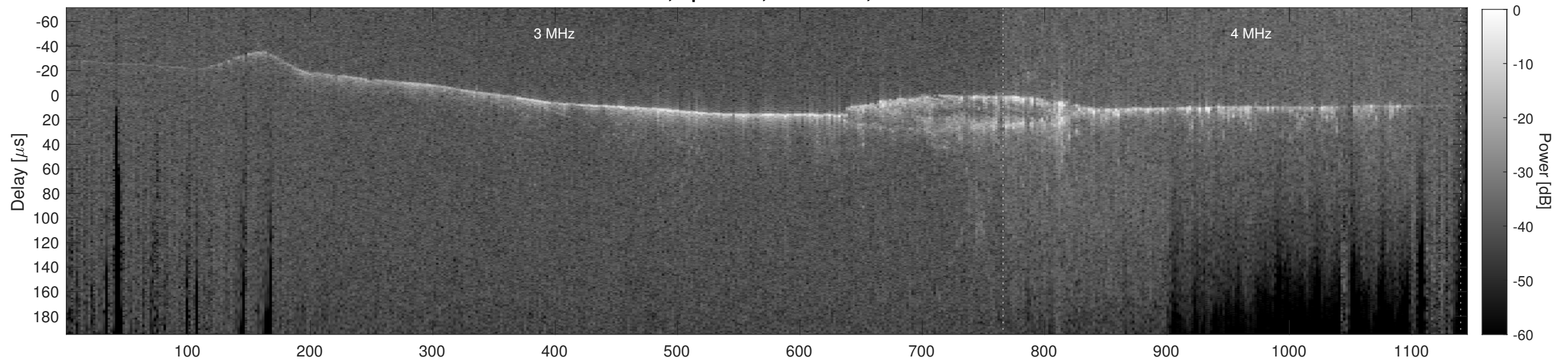
Orbit 18251, Cluttergram
