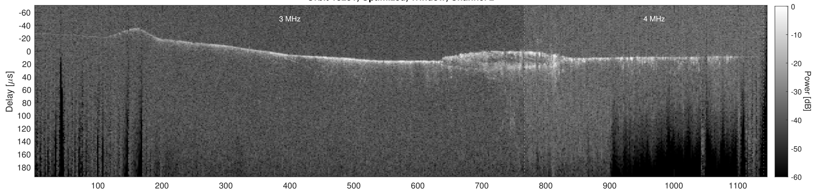
Orbit 18251, Cluttergram
