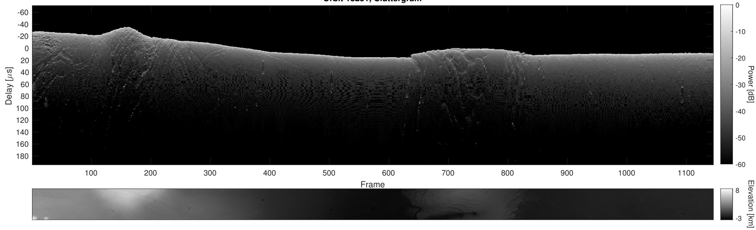
Orbit 18251, Cluttergram
