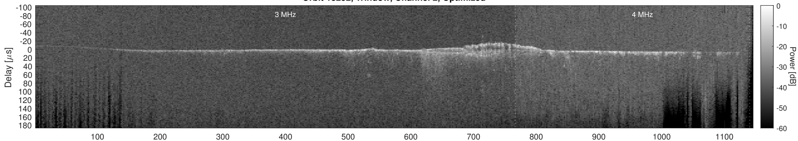
Orbit 18252, Cluttergram
