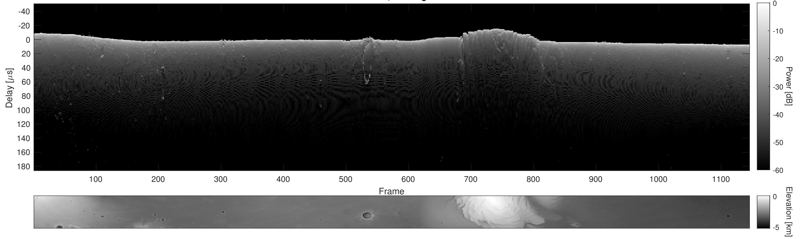
Orbit 18252, Cluttergram
