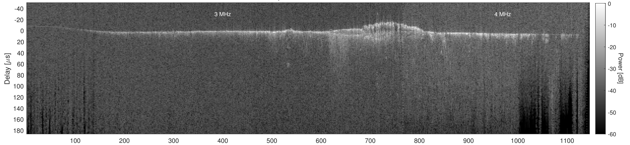
Orbit 18252, Cluttergram
