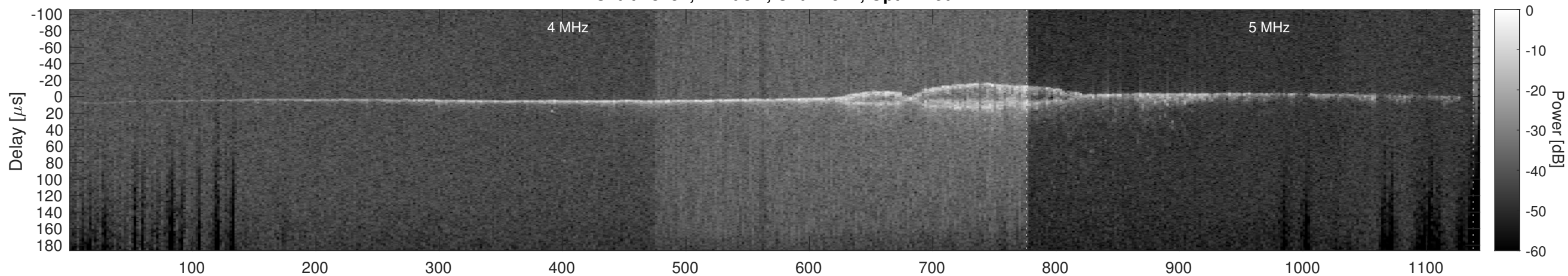
Orbit 18254, Cluttergram
