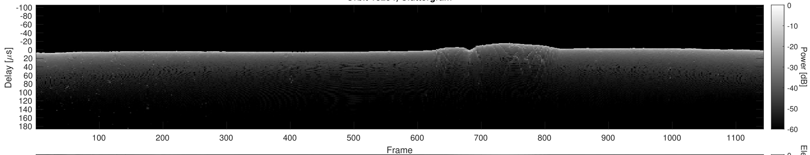
Orbit 18254, Cluttergram
