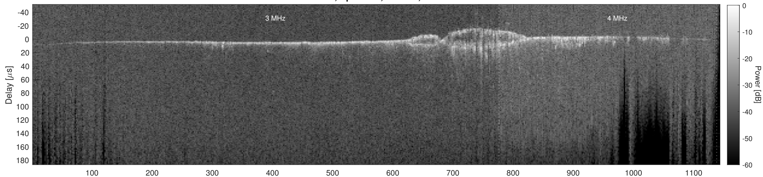
Orbit 18254, Cluttergram
