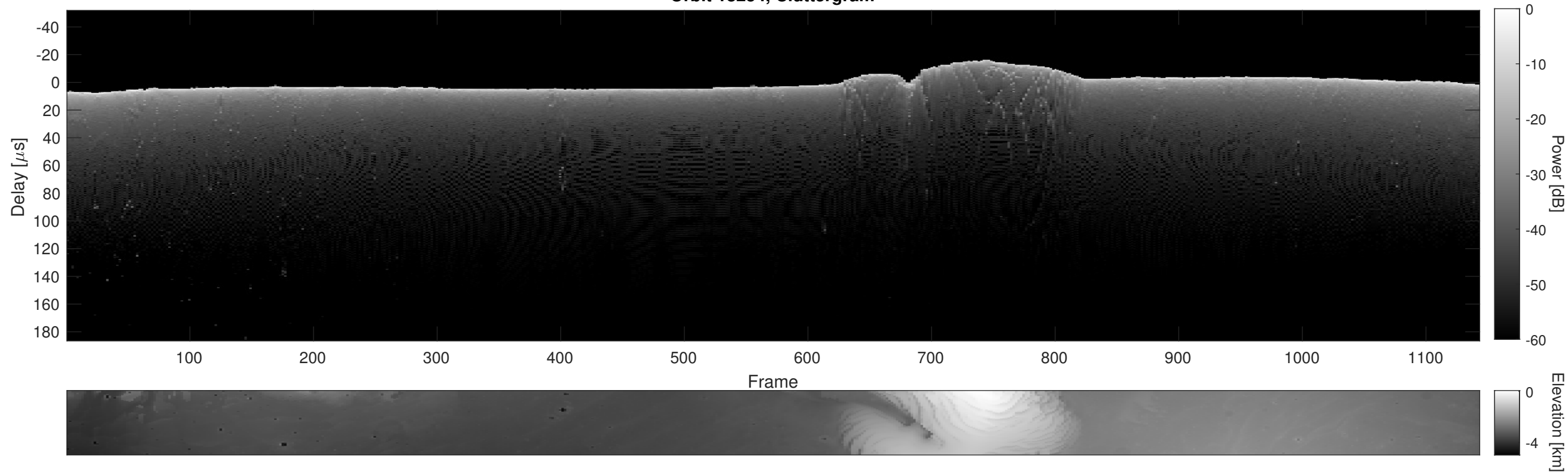
Orbit 18254, Cluttergram
