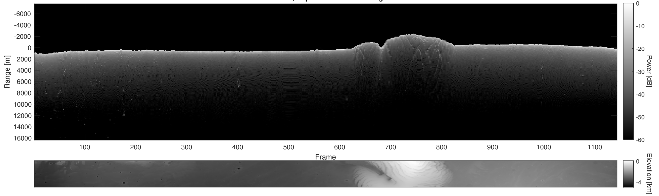
Orbit 18254, Depth-Corrected Cluttergram
