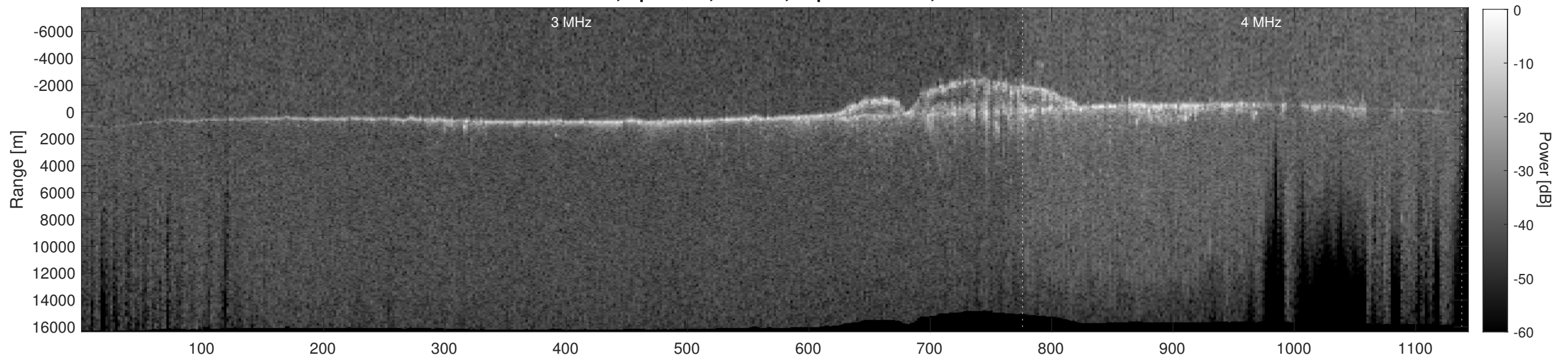
Orbit 18254, Depth-Corrected Cluttergram
