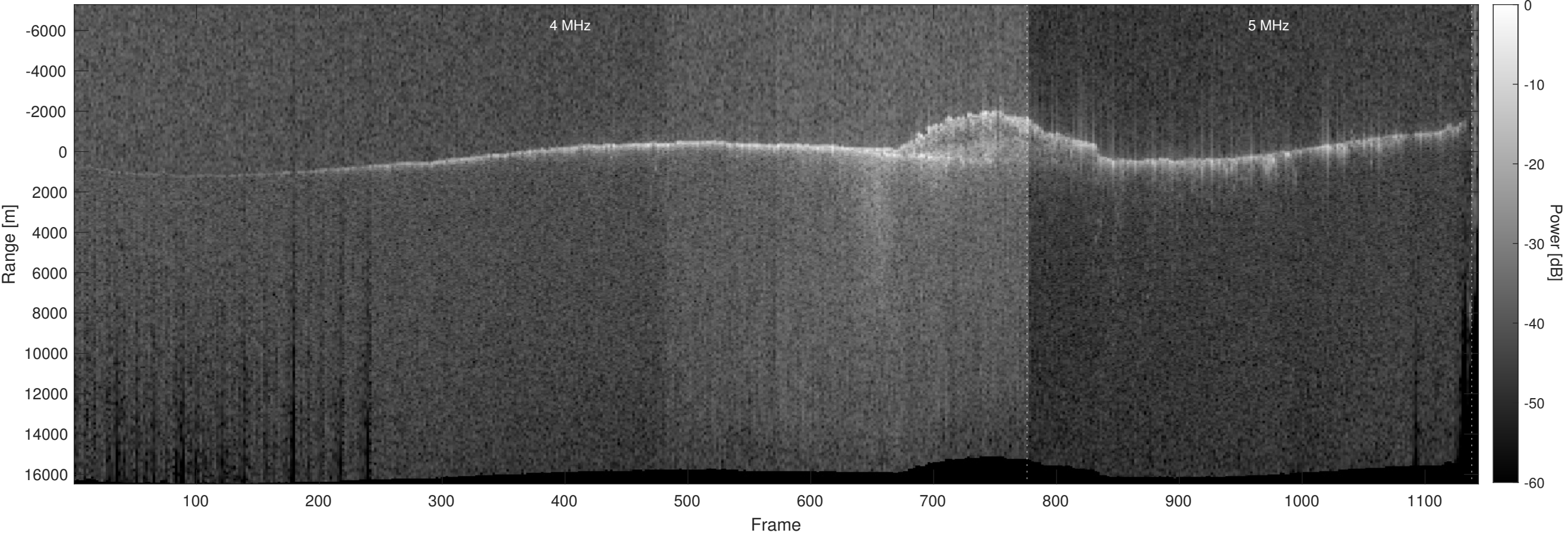
Orbit 18256, Optimized, No Window, Depth-Corrected, Channel 2
