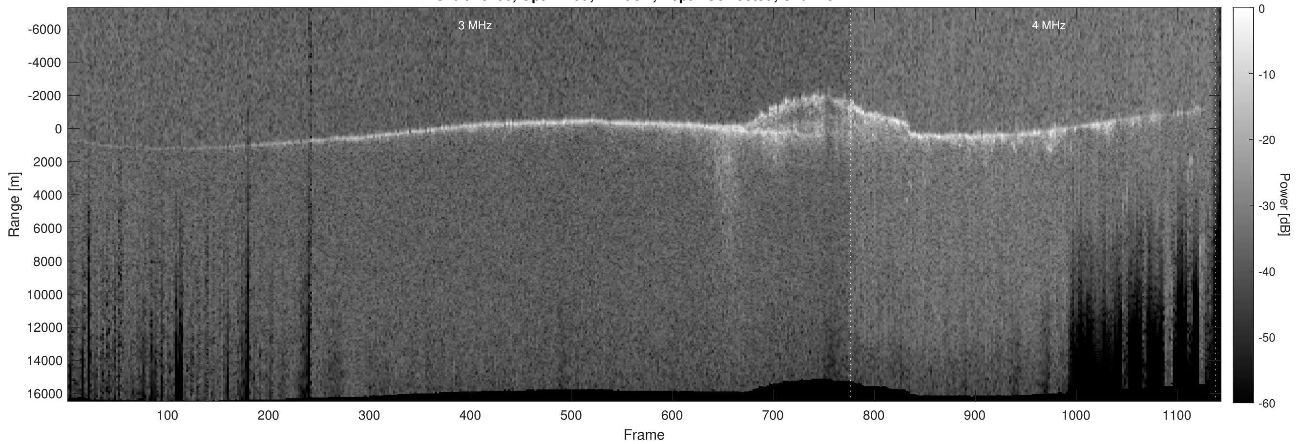
Orbit 18256, Optimized, Window, Depth-Corrected, Channel 2
