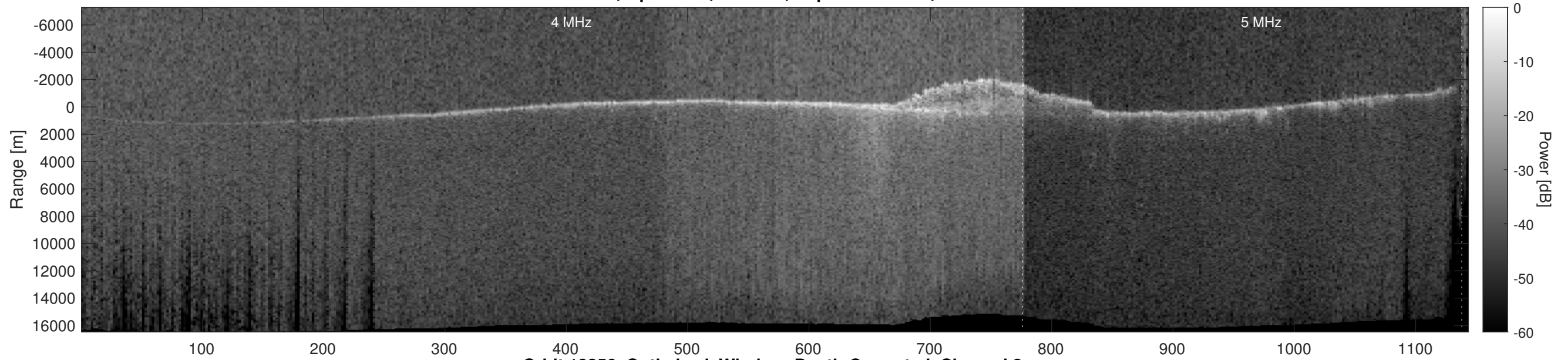
Orbit 18256, Optimized, Window, Depth-Corrected, Channel 2
