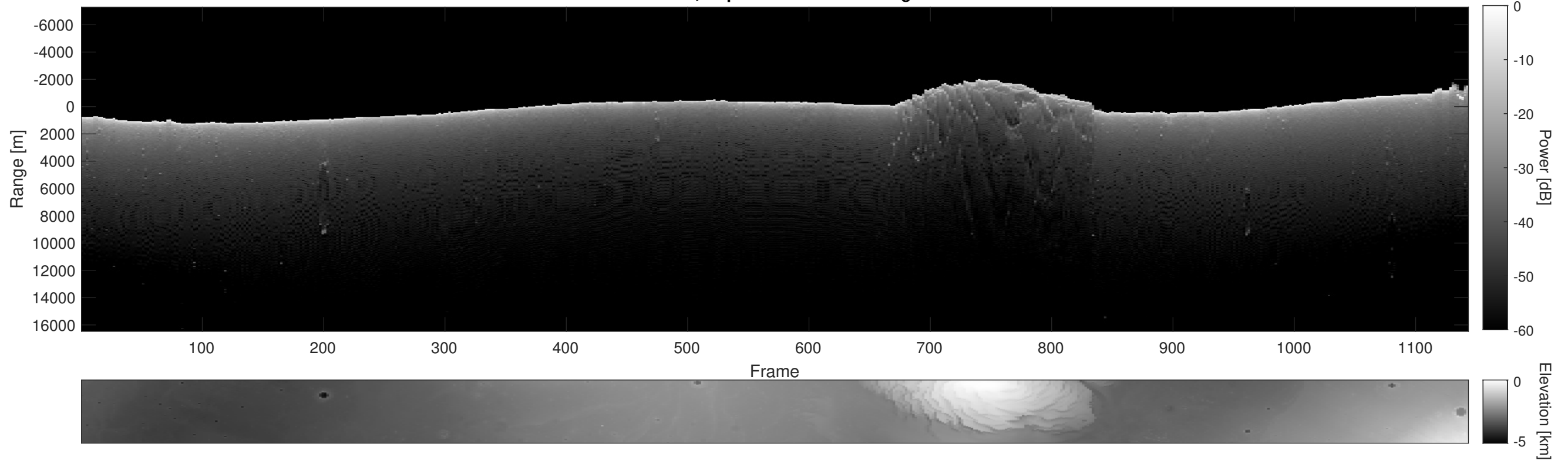
Orbit 18256, Depth-Corrected Cluttergram
