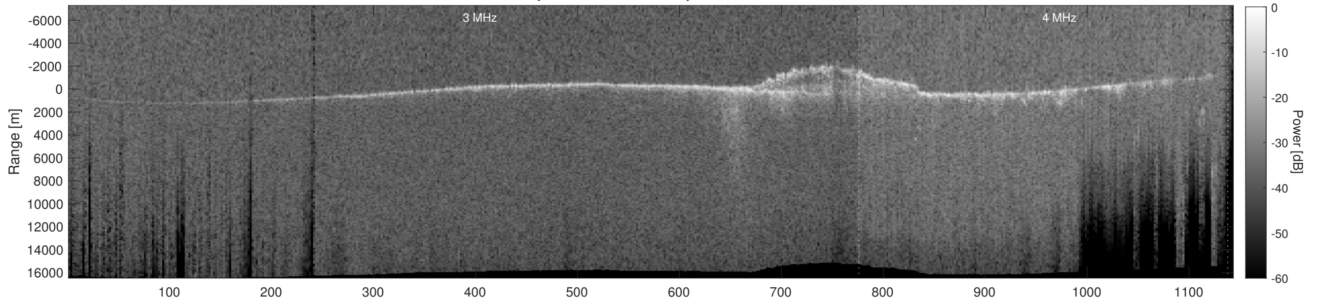
Orbit 18256, Depth-Corrected Cluttergram
