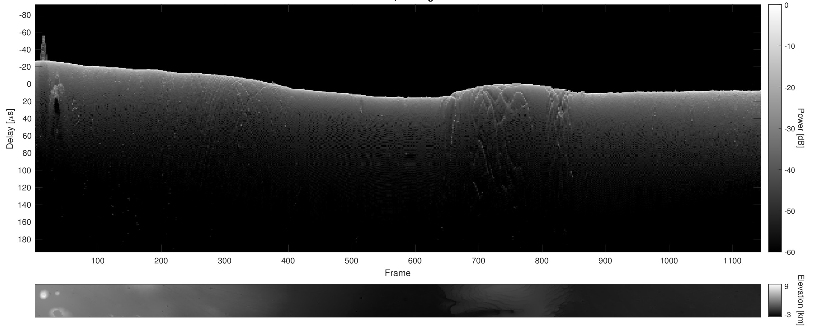
Orbit 18258, Cluttergram
