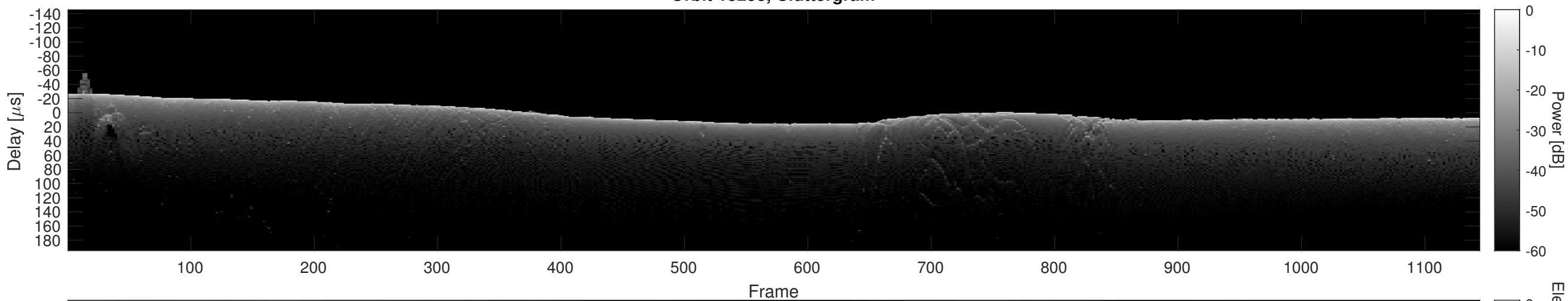
Orbit 18258, Cluttergram
