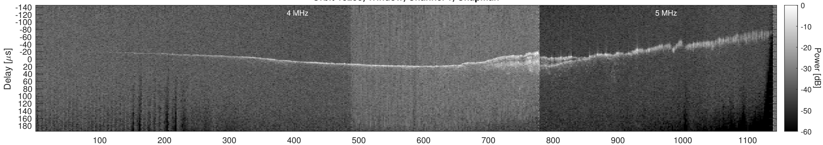
Orbit 18258, Window, Channel 1, Optimized
