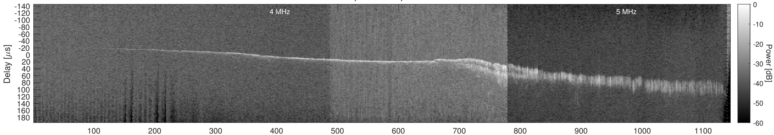
Orbit 18258, Window, Channel 1, Chapman
