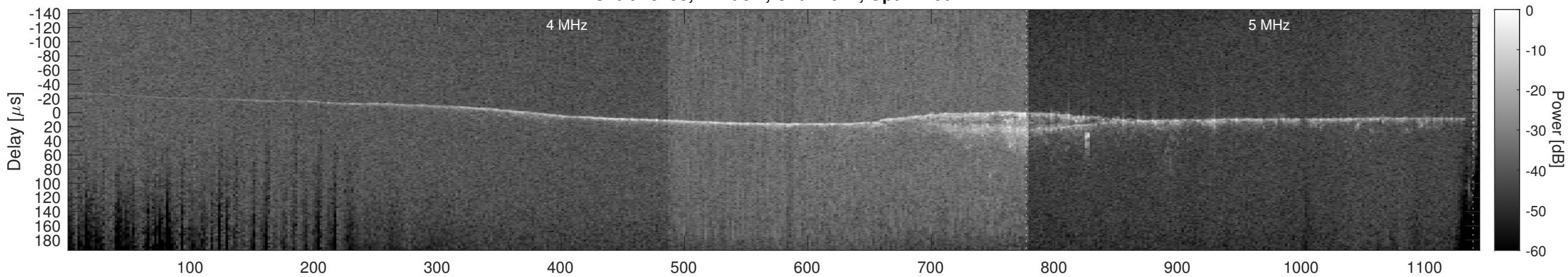
Orbit 18258, Cluttergram
