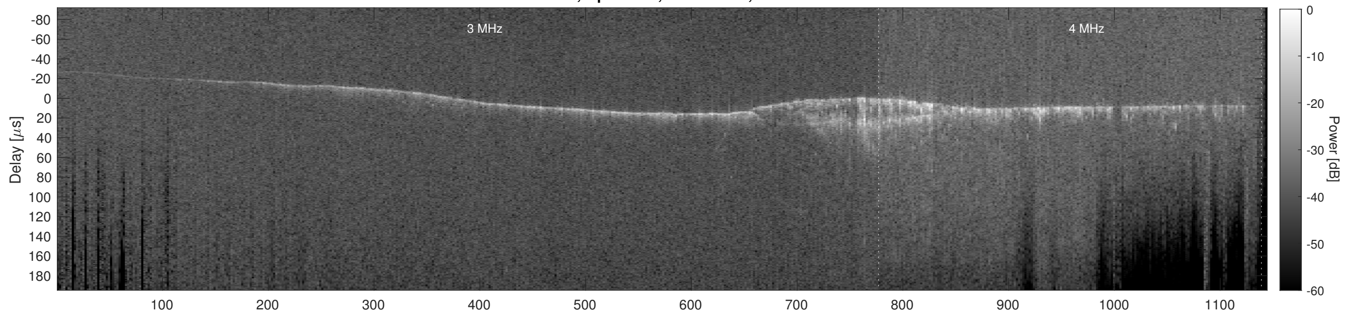
Orbit 18258, Cluttergram
