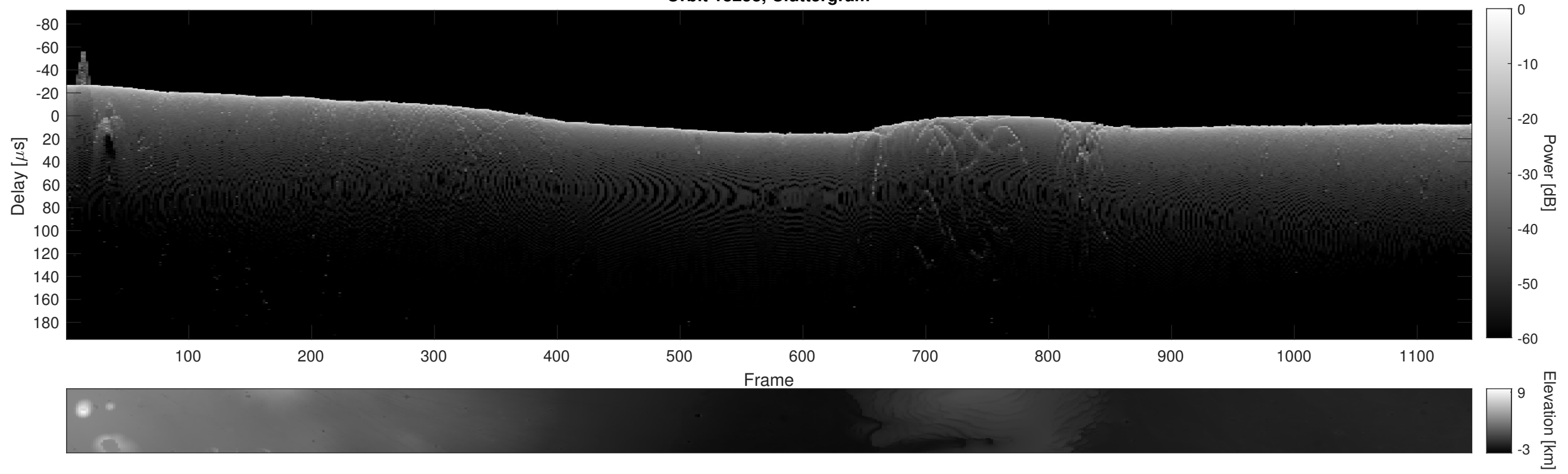
Orbit 18258, Cluttergram
