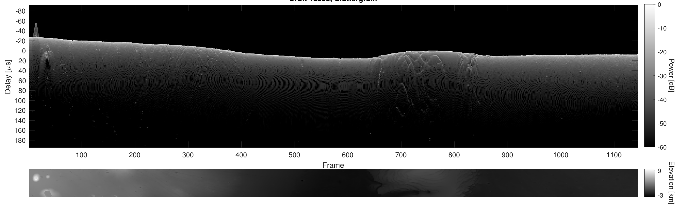
Orbit 18258, Cluttergram
