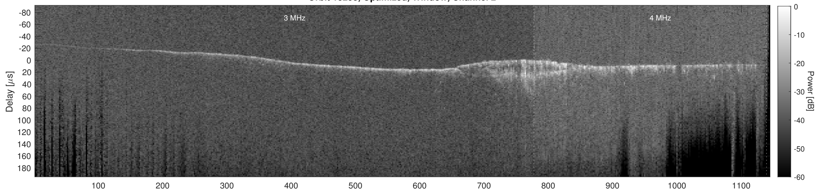
Orbit 18258, Cluttergram
