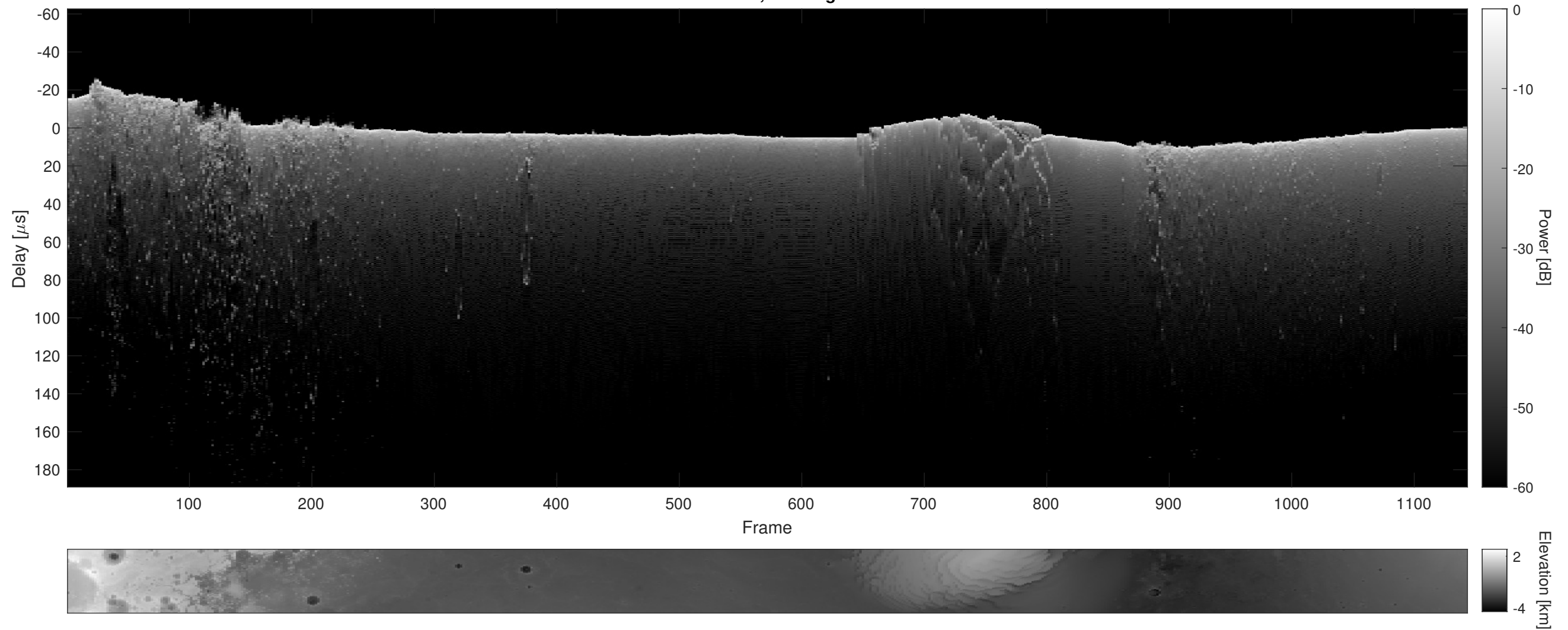
Orbit 18260, Cluttergram
