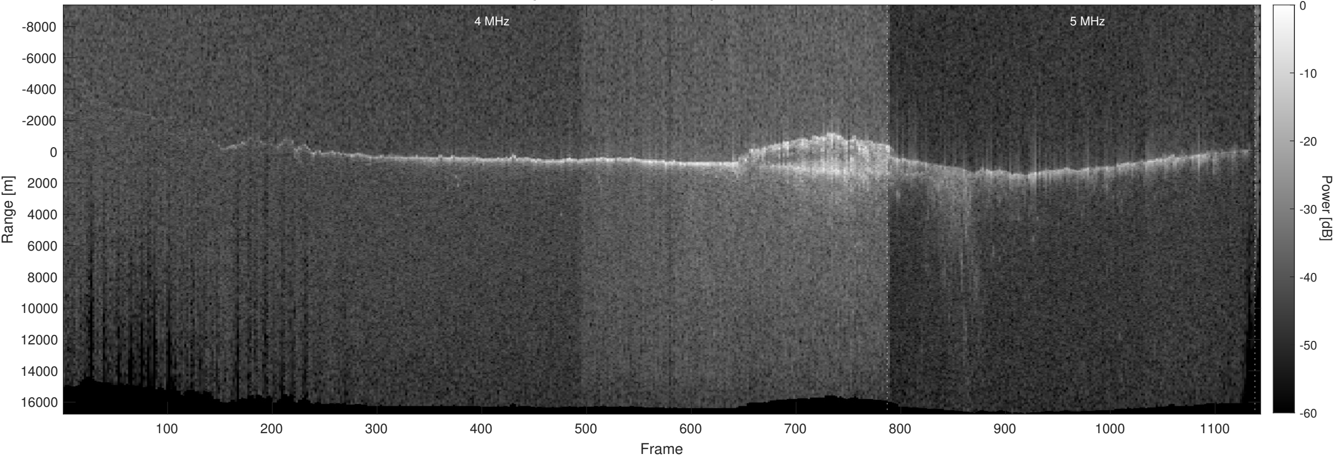
Orbit 18260, Optimized, No Window, Depth-Corrected, Channel 2
