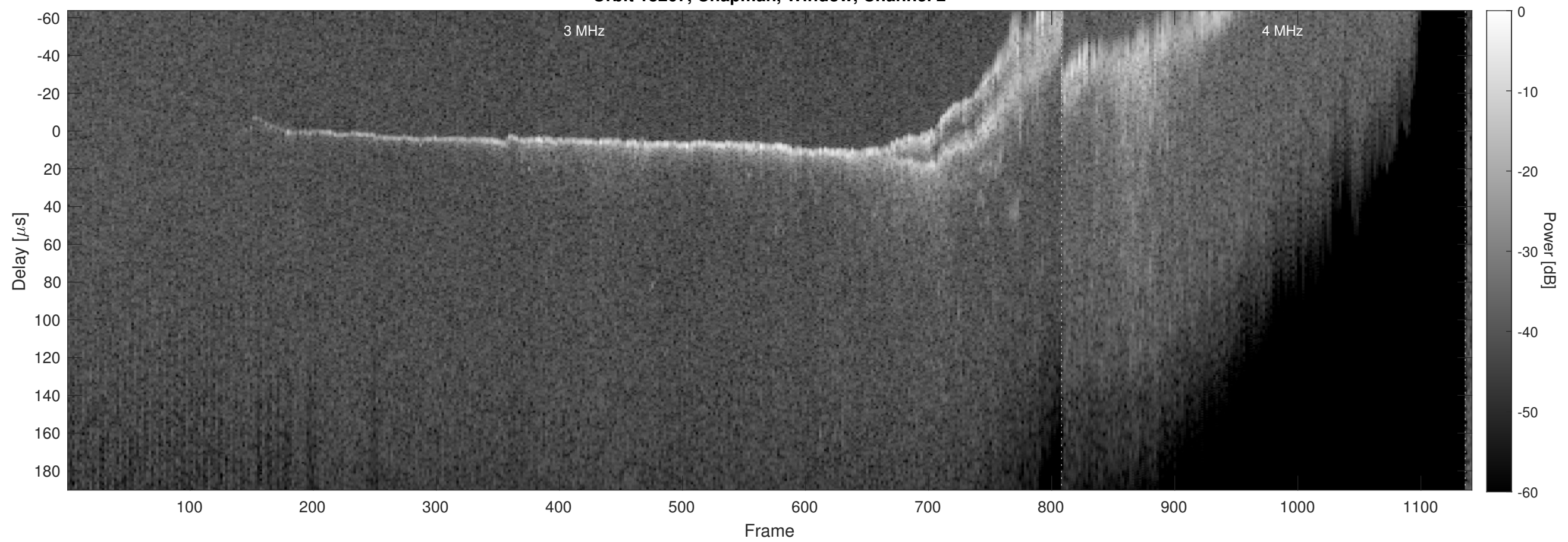
Orbit 18267, Chapman, Window, Channel 2
