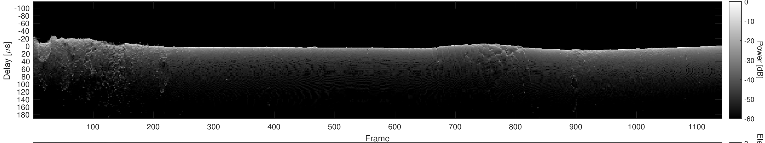
Orbit 18267, Cluttergram
