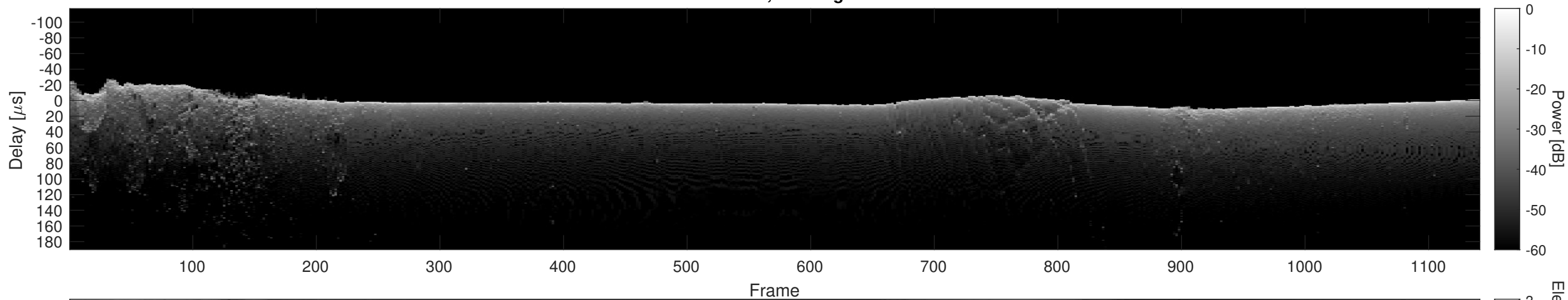
Orbit 18267, Cluttergram
