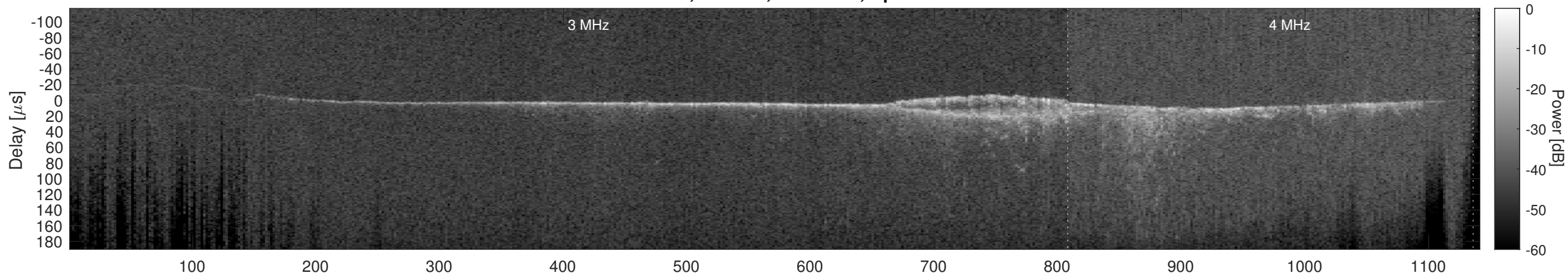
Orbit 18267, Cluttergram
