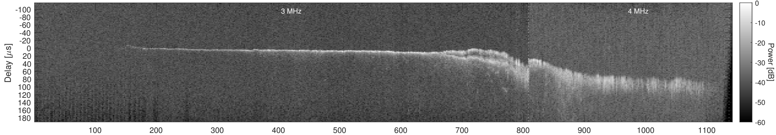
Orbit 18267, Window, Channel 2, Chapman
