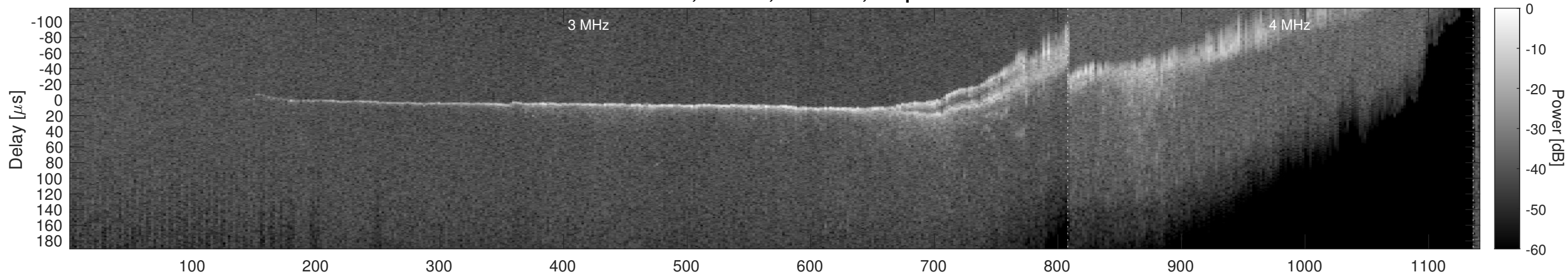
Orbit 18267, Window, Channel 2, Optimized
