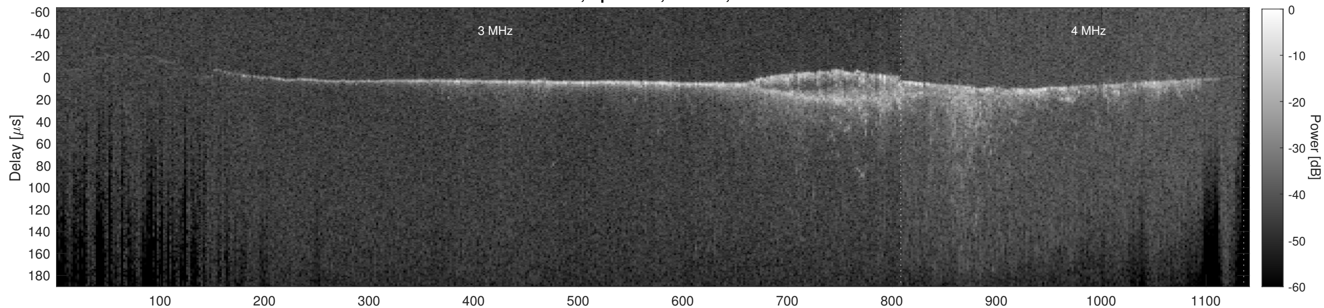
Orbit 18267, Cluttergram
