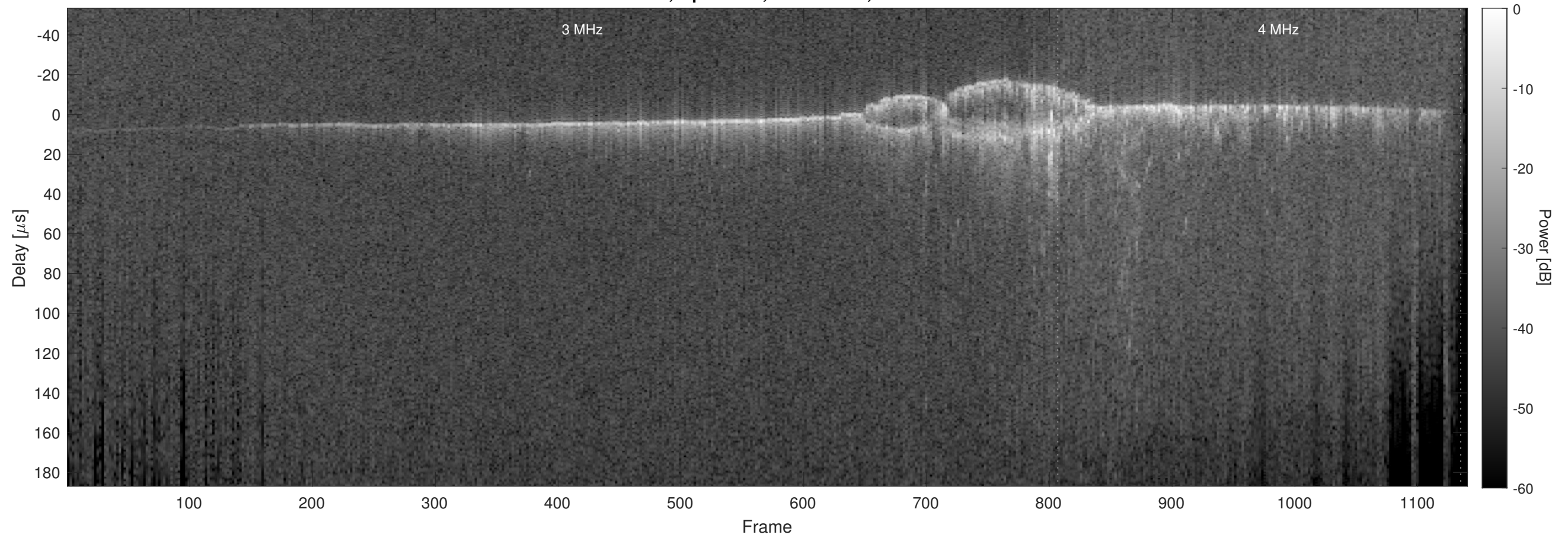
Orbit 18268, Optimized, No Window, Channel 2
