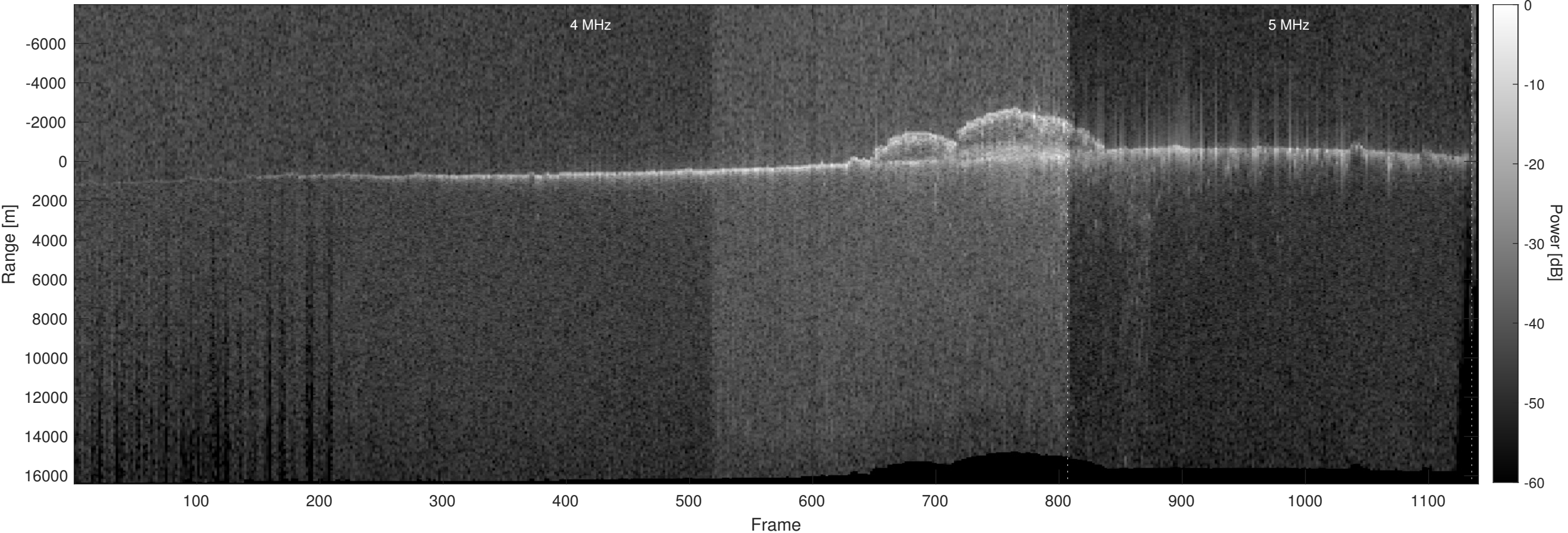
Orbit 18268, Optimized, No Window, Depth-Corrected, Channel 2
