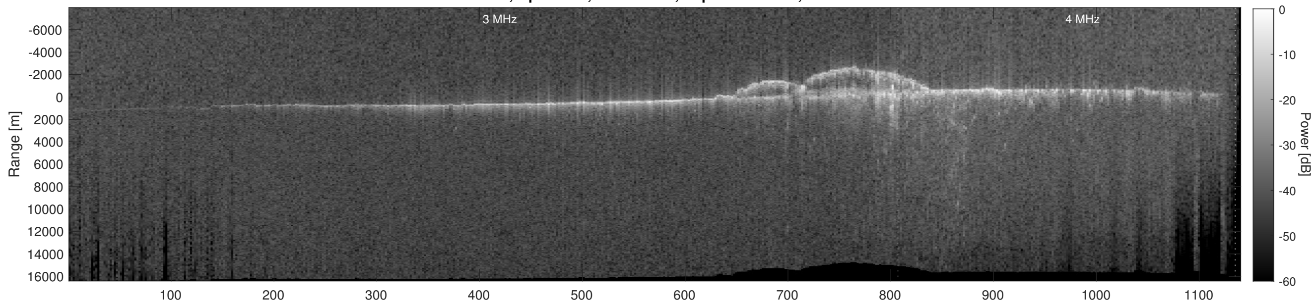
Orbit 18268, Depth-Corrected Cluttergram
