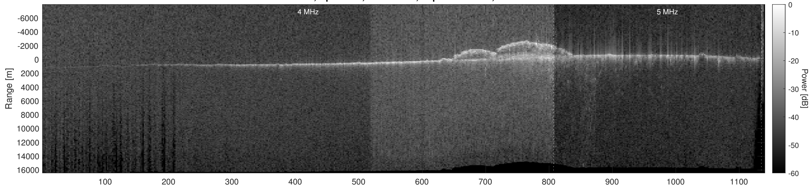
Orbit 18268, Optimized, No Window, Depth-Corrected, Channel 2
