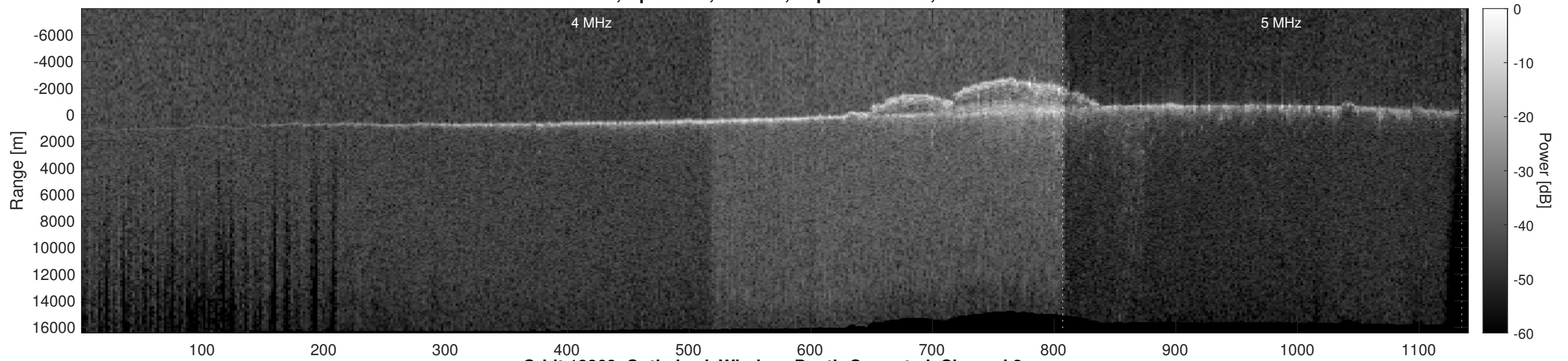
Orbit 18268, Optimized, Window, Depth-Corrected, Channel 2
