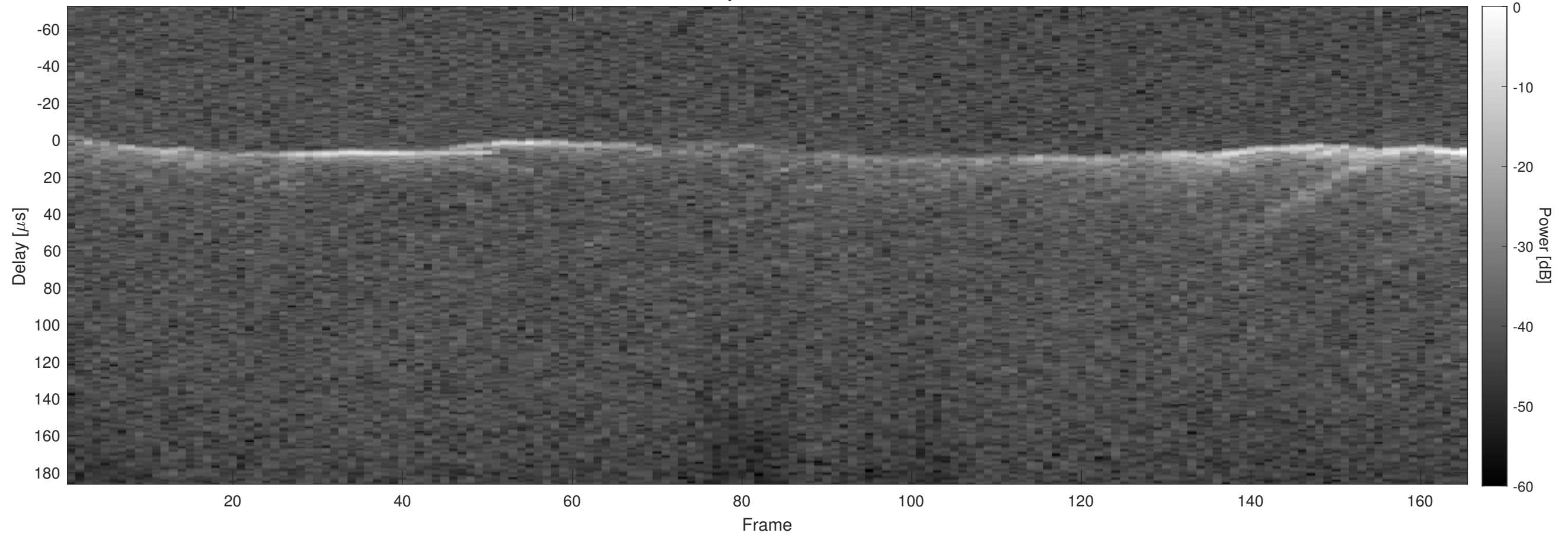
Orbit 18269, Chapman, Window, Channel 2
